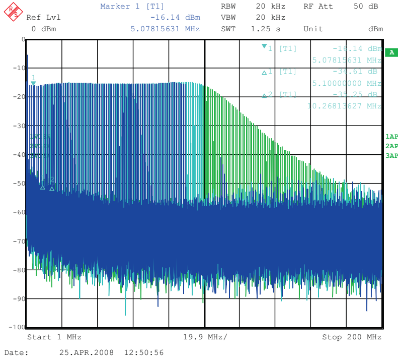
Figure 9. THS3091 and THS3095 LPF Filter Shape Evaluated With Multi-tone Input Signal From the TSW3100 Pattern Generator
