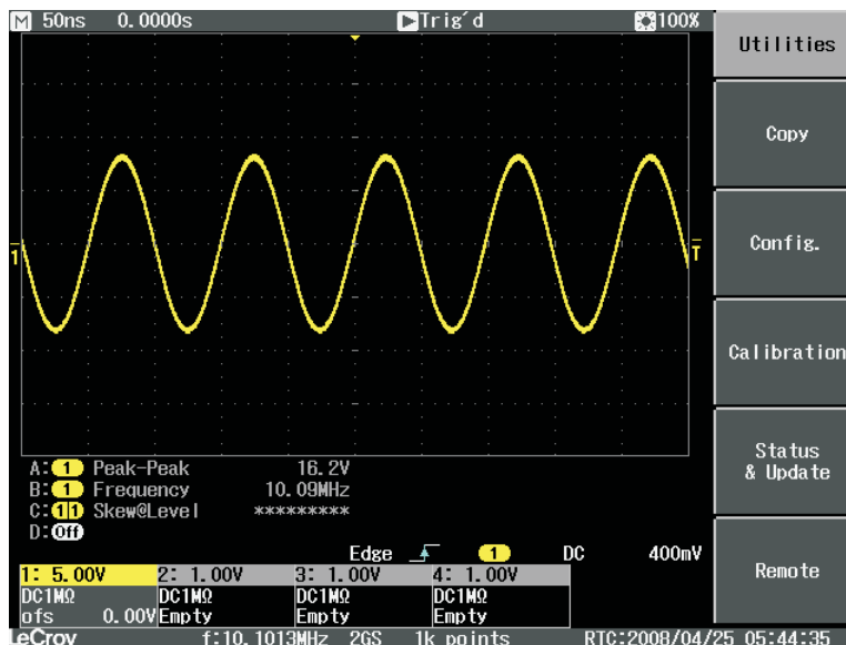
Figure 8. THS3091 and THS3095 With ±15-V External Supplies, 50-Ω Input, Gain at 10x
