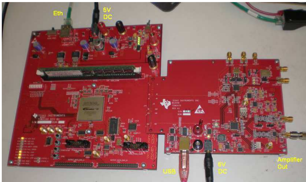
Figure 6. TSW3070EVM Driven by TSW3100 Pattern Generator
