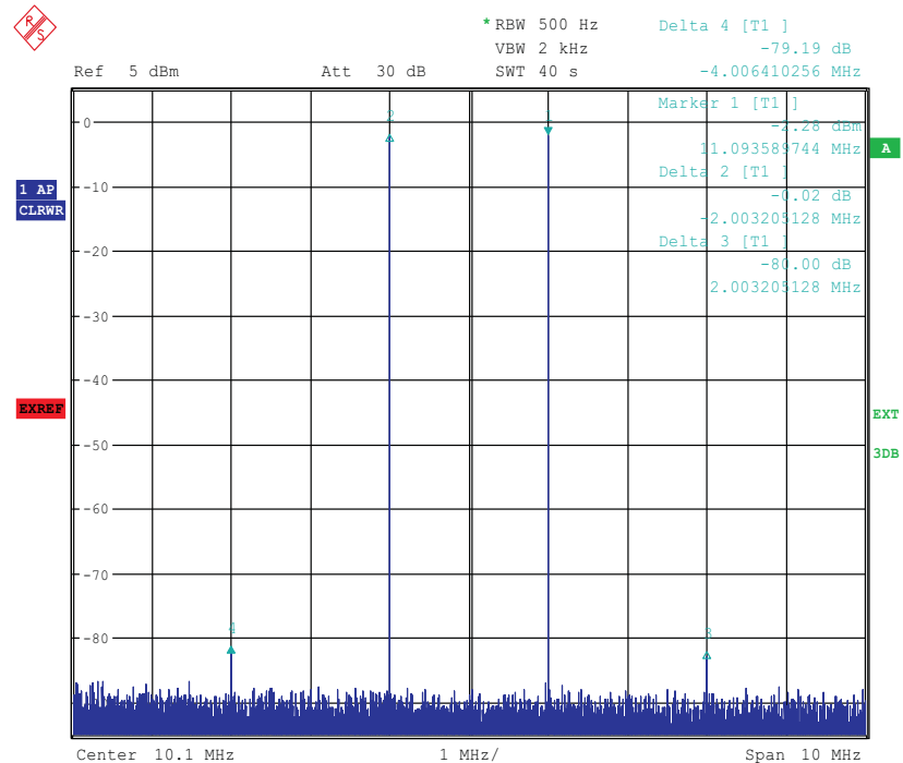
Figure 11. IMD3 Plot for THS3095
