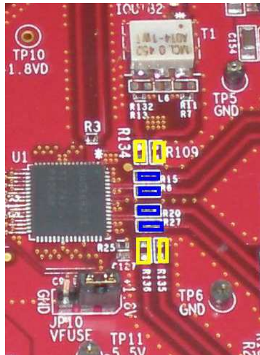
Figure 17. DAC5682Z Resistor Jumper Configuration
