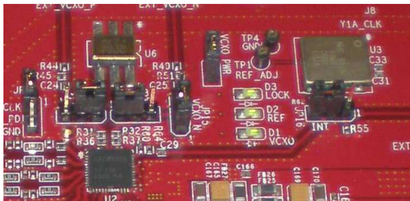
Figure 15. CDCM7005, 800M VCXO, 10M Ref, Locked Condition LEDs
