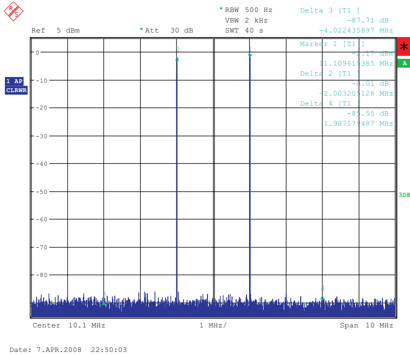
Figure 12. IMD3 Plot for OPA695
