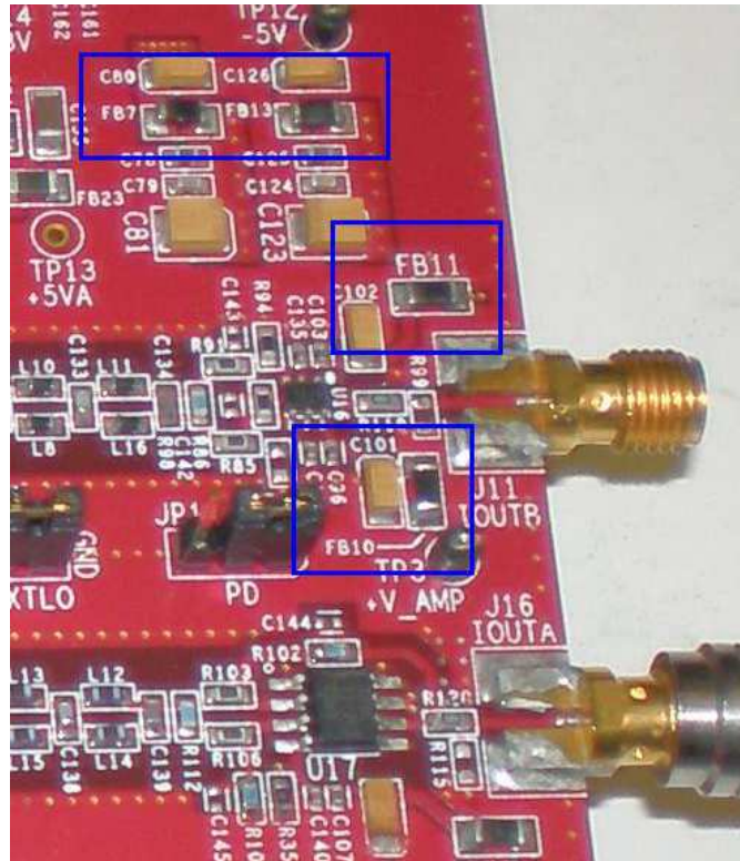
Figure 18. Position of Ferrite Beads for Power Options
