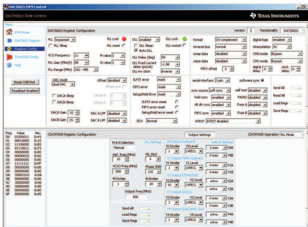
Figure 16. DAC5682 and CDCM7005 Example Register Settings
