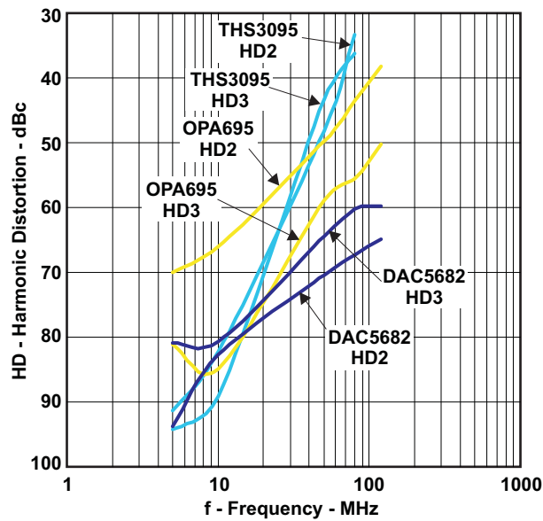
Figure 14. Summary of Harmonic Distortion for Passive Transformer, OPA695, THS3091, and THS3095 Output
