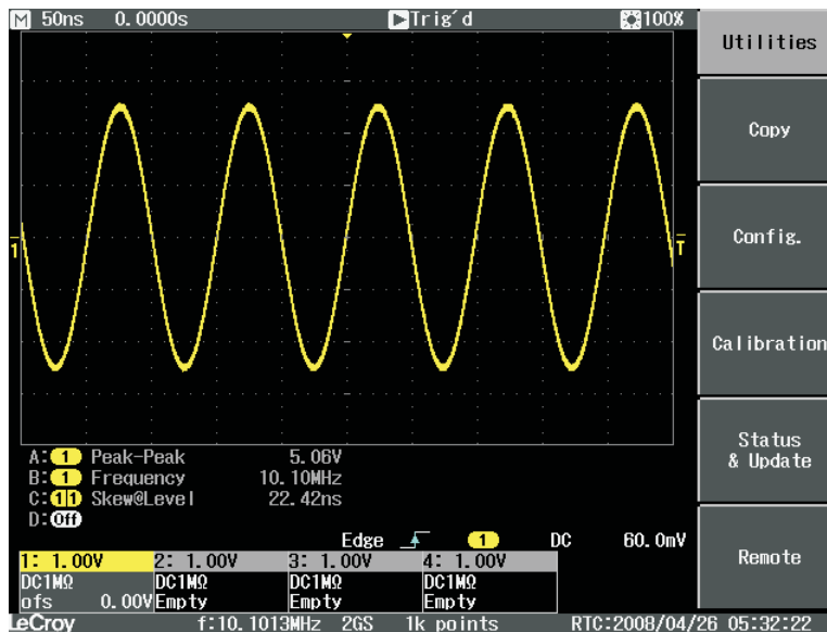
Figure 7. Typical THS3091 and THS3095 Voltage Output, Default Gain 3.3x
