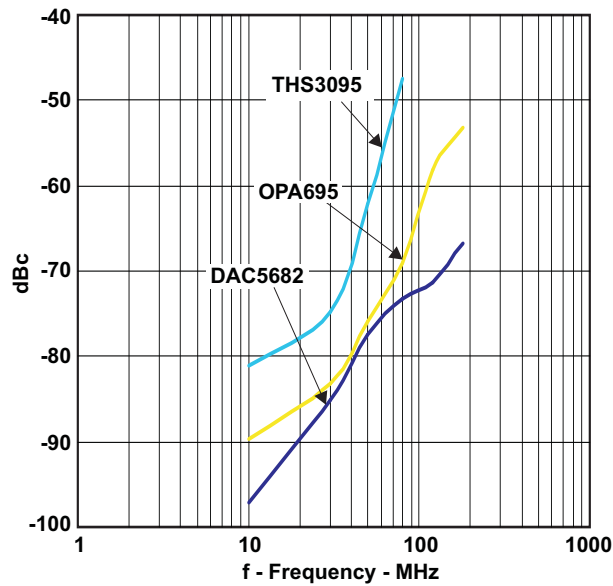
Figure 13. Summary of IMD3 for Passive Transformer, OPA695, THS3091, and THS3095 Output
