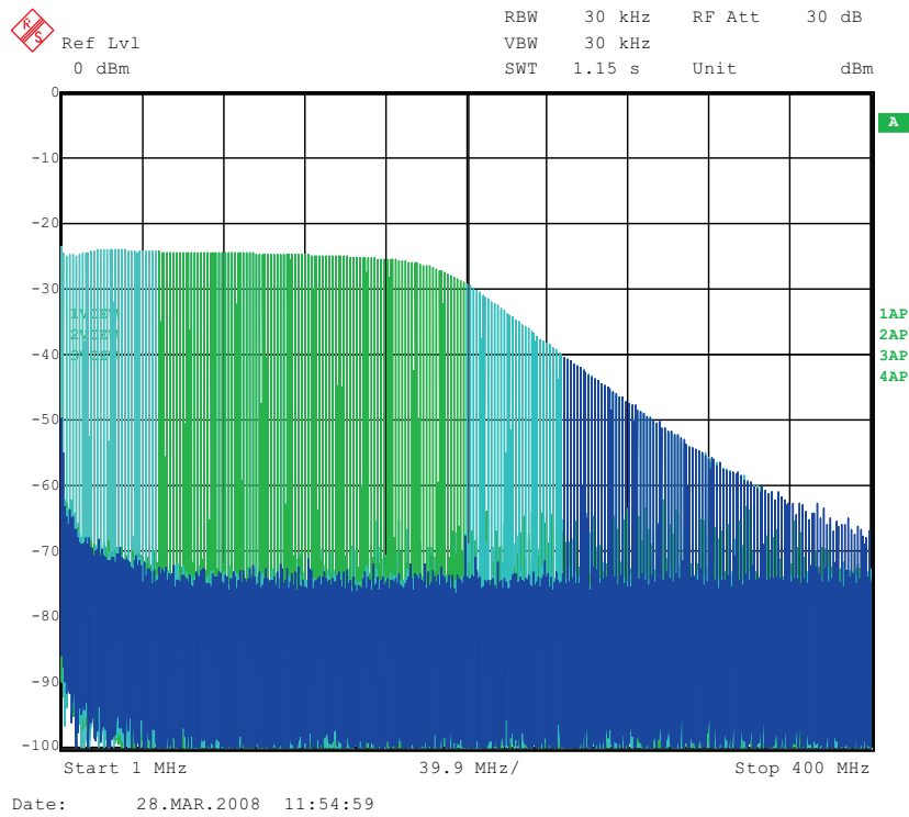
Figure 10. OPA695 LPF Filter Shape Evaluated With Multi-tone Signal
