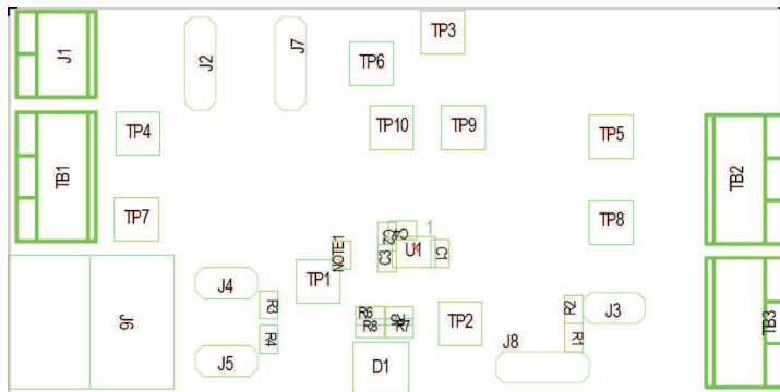
Figure 2. bq27425EVM Layout – Top Assembly
