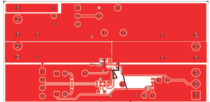
Figure 3. bq27425EVM Layout – Top Layer
