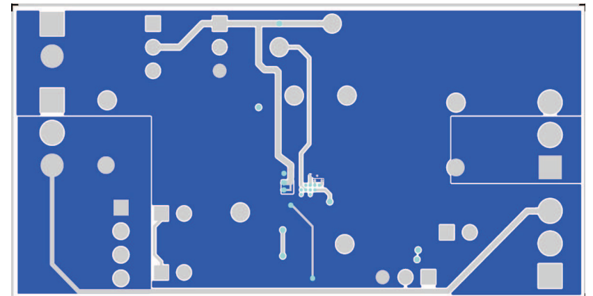
Figure 4. bq27425EVM Layout – Bottom Layer
