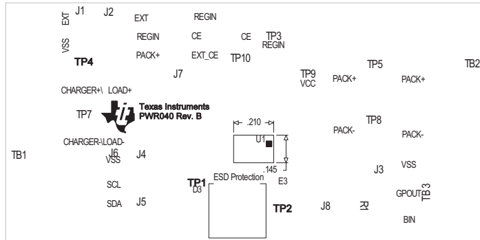
Figure 1. bq27425EVM Layout – Top Silk
