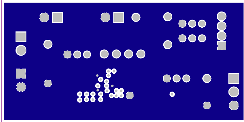
Figure 5. bq27421EVM Layout – Ground Layer
