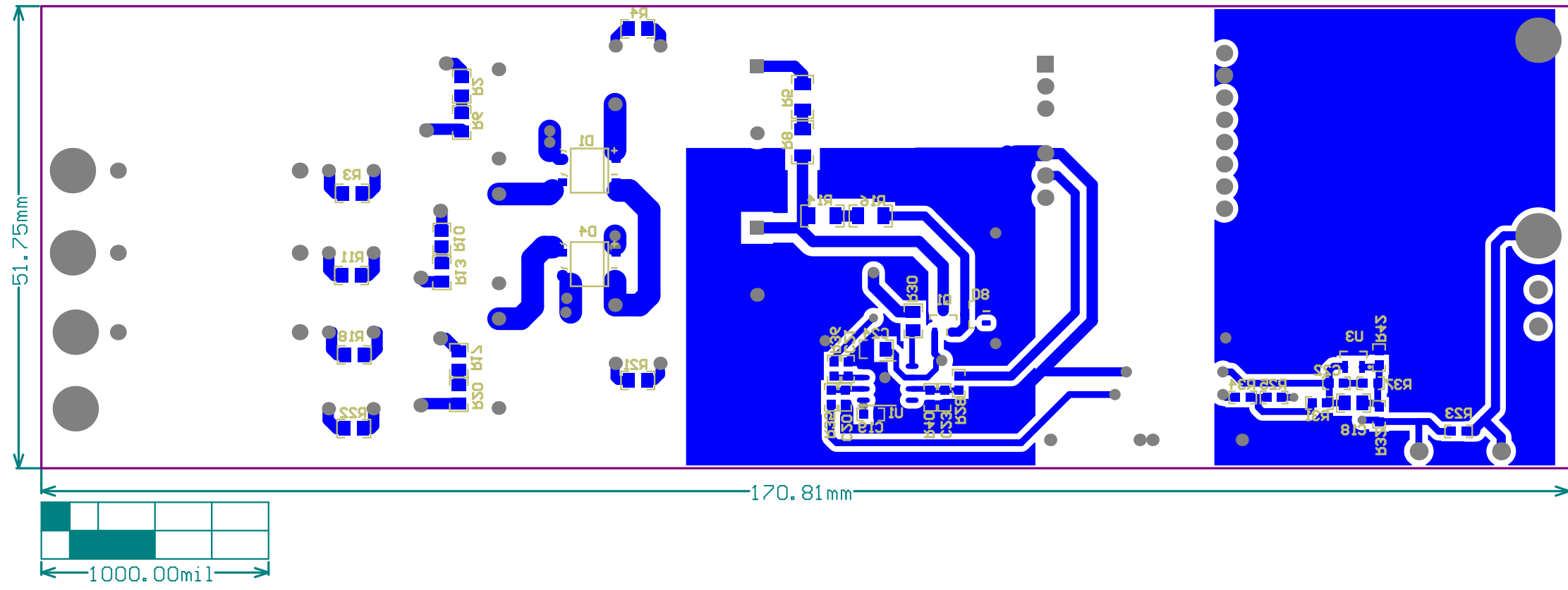
PCB Board Dimensions
