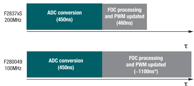
Figure 4. A comparison of FCL execution on the F2837x and F28004x.
