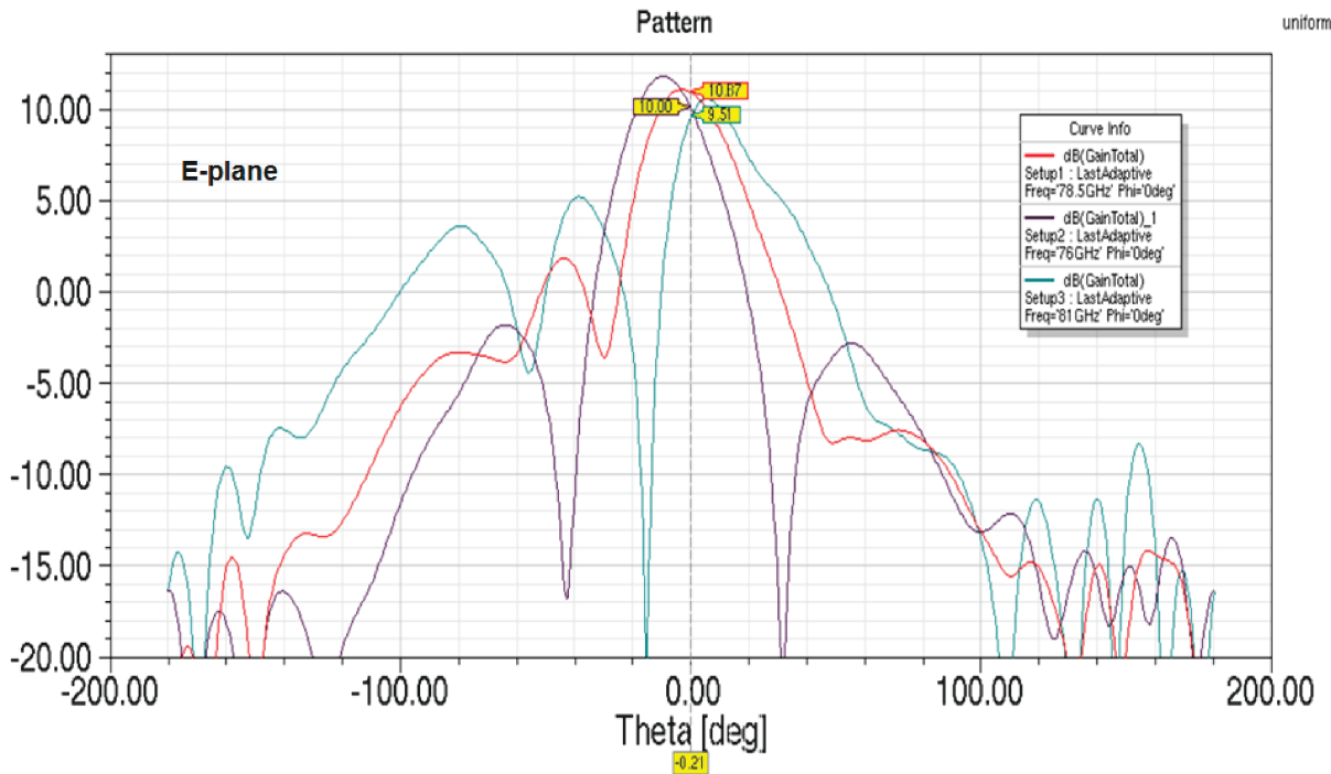
Figure 2-11. Antenna Pattern in E-Plane
