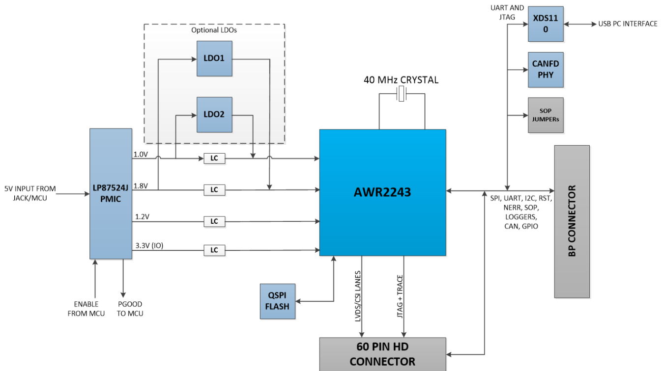
Figure 2-3. BoosterPack™ Block Diagram
