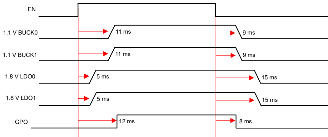
Figure 3-1. LP873245-Q1 Power-up and Power Down Sequence
