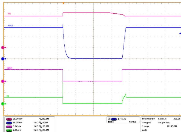
Figure 3-6. Overvoltage Lockout Response of TPS1685 eFuse ( V_{IN} Ramped Up from 54V to 62V and Ramped Down to 54V, V_{IN(OVP)}=60V , C_{OUT} = 1mF , and R_{LOAD} = 50\Omega )
