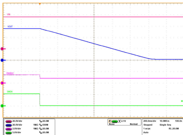
Figure 3-11. QOD Enabled on TPS1685 eFuse ( V_{IN} = 54V , C_{OUT} = 1mF , and EN Pulled Low to 1V)
