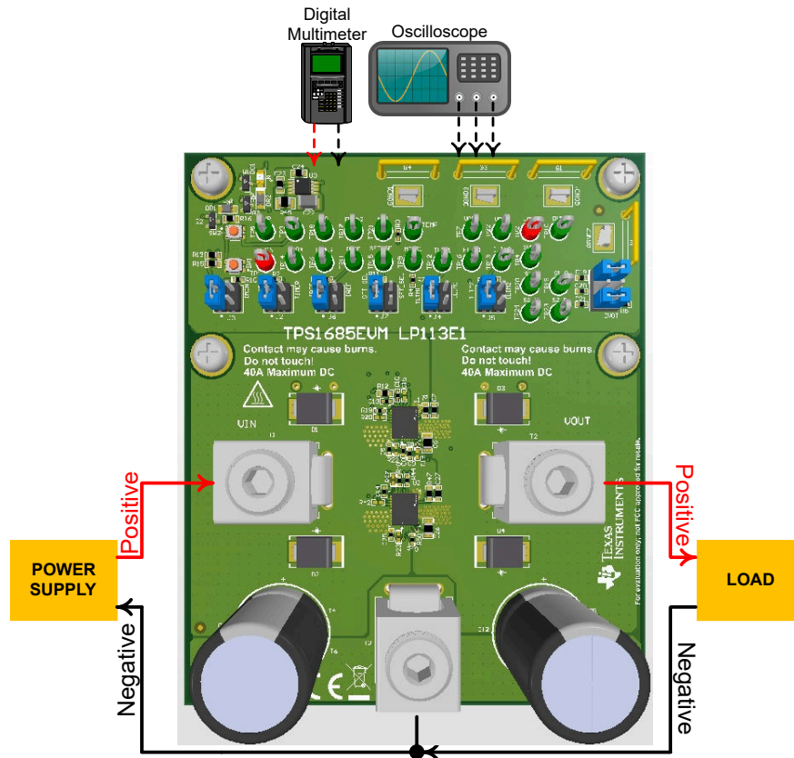
Figure 3-1. TPS1685EVM Setup with Test Equipment
