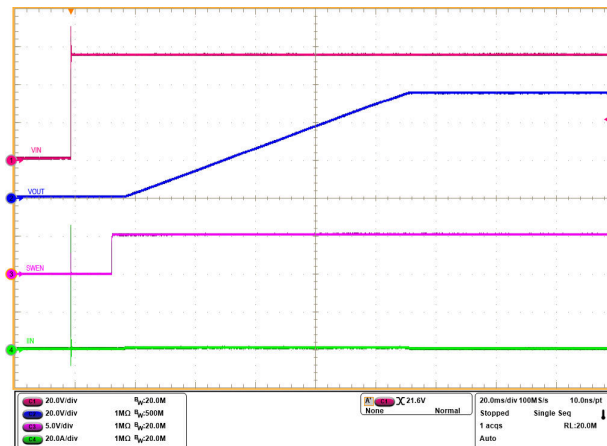
Figure 3-2. TPS1685 eFuse Hot Plug Profile ( V_{IN} Stepped Up from 0V to 54V, C_{OUT} = 1\text{mF} , and C_{DVRT} = 82\text{nF} )
