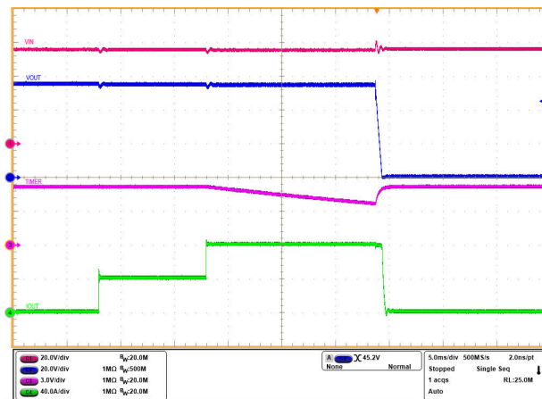
Figure 3-8. Persistent Overload Performance of TPS1685 eFuse ( V_{IN} = 54V , C_{TIMER} = 27nF , C_{OUT} = 1mF , R_{IMON} = 1.1k\Omega ( I_{OCP} = 50A ), R_{IREF} = 40.2k\Omega ( V_{REF} = 1V ), and I_{OUT} Ramped from 40A for 10ms to 80A for 20ms)
