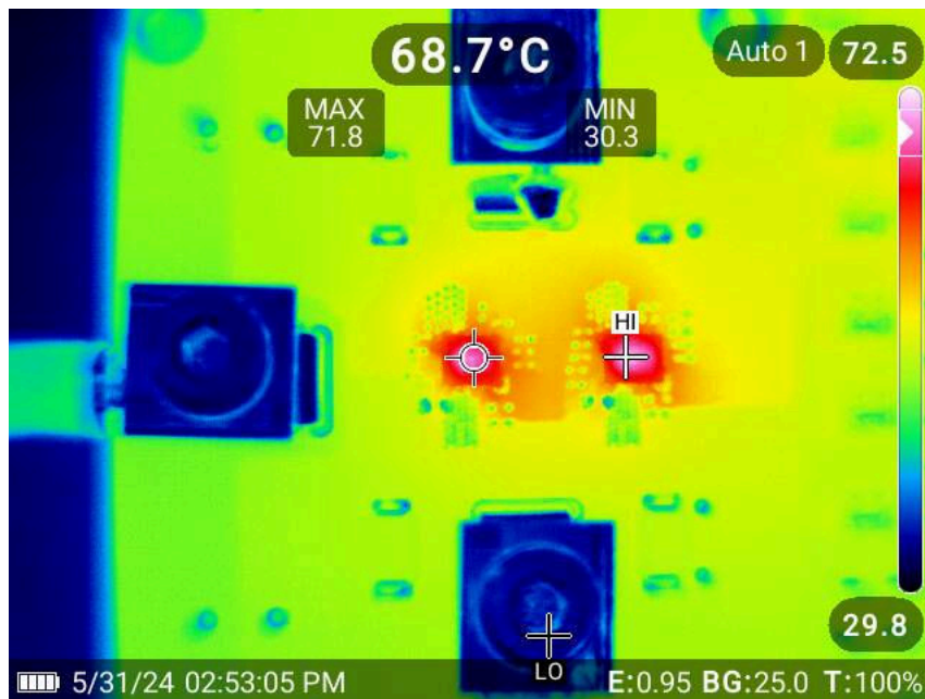
Figure 3-13. Thermal Performance of TPS1685EVM ( V_{IN} = 54V , I_{OUT} = 40A , T_A = 30^{\circ}C , and no external air flow)
