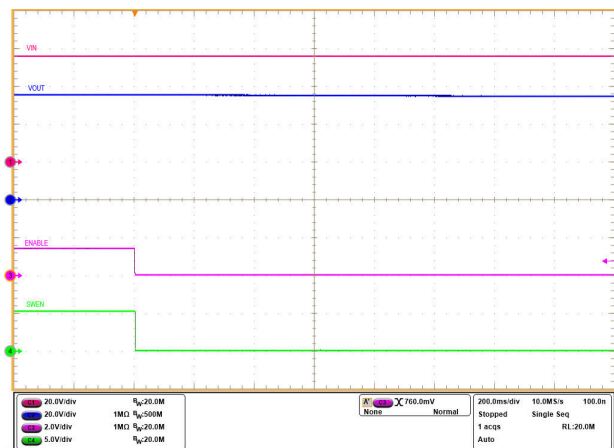
Figure 3-12. QOD Disabled on TPS1685 eFuse ( V_{IN} = 54V , C_{OUT} = 1mF , and EN Pulled Low to 0V)
