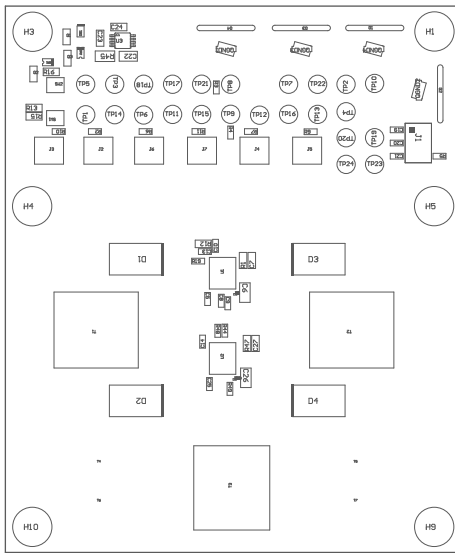
Figure 4-2. TPS1685EVM Board: Top Assembly
