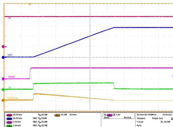
Figure 3-3. TPS1685 eFuse Start-up Profile with ENABLE ( V_{IN} = 54\text{V} , EN Stepped Up from 0V to 5V, C_{OUT} = 1\text{mF} , and C_{DVRT} = 82\text{nF} )
