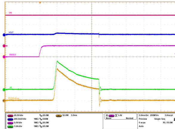
Figure 3-4. Power Up into Output Short Response of TPS1685 eFuse ( V_{IN} = 54V , EN Stepped Up from 0V to 5V, and OUT Shorted to PGND)
