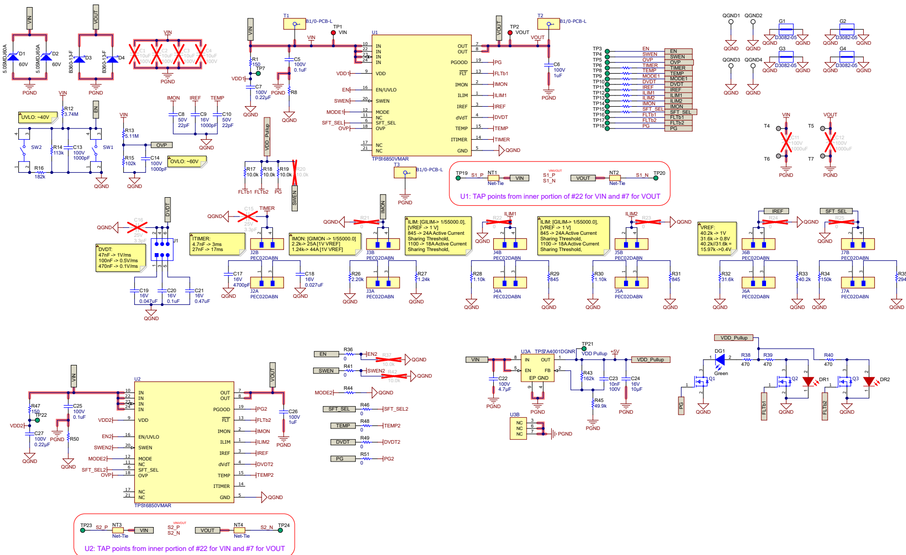
Figure 4-1. TPS1685EVMFuse Evaluation Board Schematic
