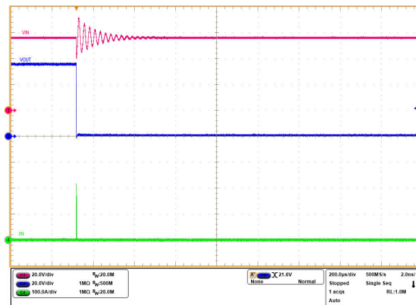
Figure 3-9. Output Hot Short Response (zoomed out) in TPS1685EVM ( V_{IN} = 54V , R_{IMON} = 1.1k\Omega , R_{IREF} = 40.2k\Omega , R_{SFT} = 150k\Omega , and C_{OUT} = 1mF )
