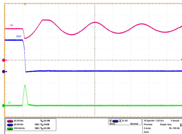
Figure 3-10. Output Hot Short Response (zoomed in) in TPS1685EVM ( V_{IN} = 54V , R_{IMON} = 1.1k\Omega , R_{IREF} = 40.2k\Omega , R_{SFT} = 150k\Omega , and C_{OUT} = 1mF )
