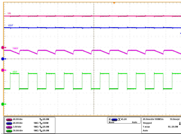
Figure 3-7. Transient Overload Performance of TPS1685 eFuse ( V_{IN} = 54V , C_{TIMER} = 27nF , C_{OUT} = 1mF , R_{IMON} = 1.1k\Omega ( I_{OCP} = 50A ), R_{IREF} = 40.2k\Omega ( V_{REF} = 1V ), and I_{OUT} Ramped from 40A for 10ms to 80A for 10ms)
