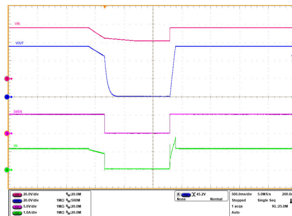
Figure 3-5. Undervoltage Lockout Response of TPS1685 eFuse ( V_{IN} Ramped Down from 54V to 38V and Ramped Up to 54V, V_{IN(UVP)}=40V , C_{OUT} = 1mF , and R_{LOAD} = 50\Omega )
