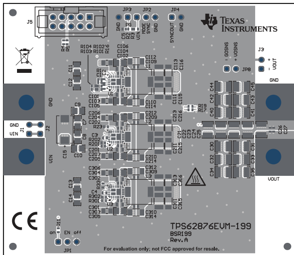
Figure 5-1. Top Layer - Components
