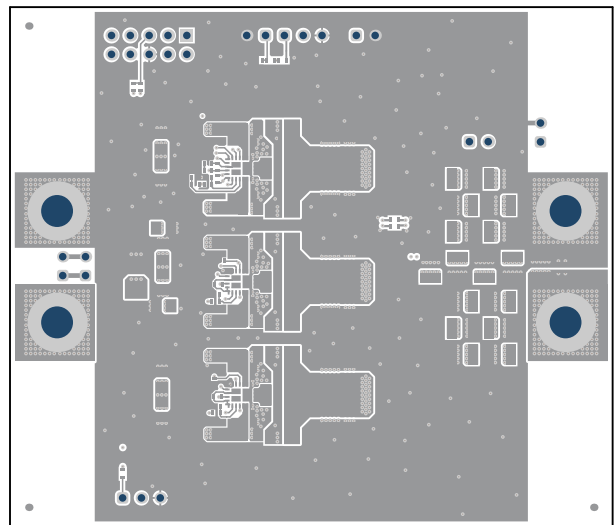
Figure 5-2. Top Layer
