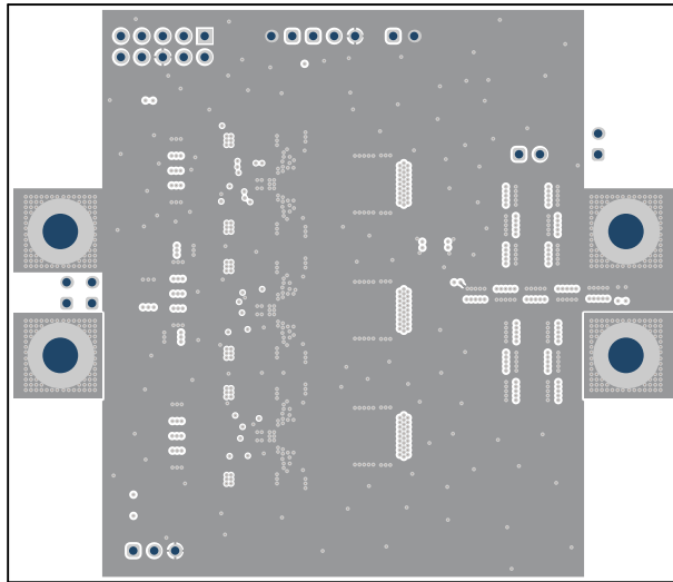
Figure 5-3. Layer 2
