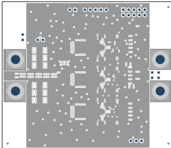
Figure 5-11. Bottom Layer
