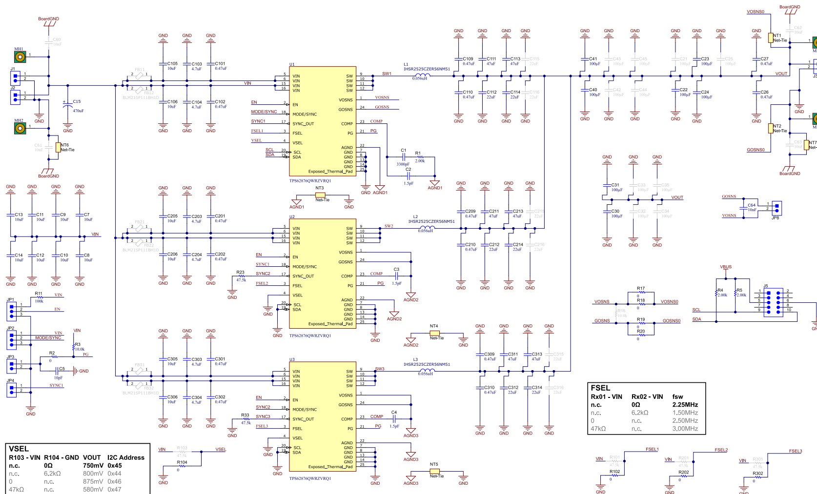
Figure 6-1. TPS62876EVM-199 Schematic
