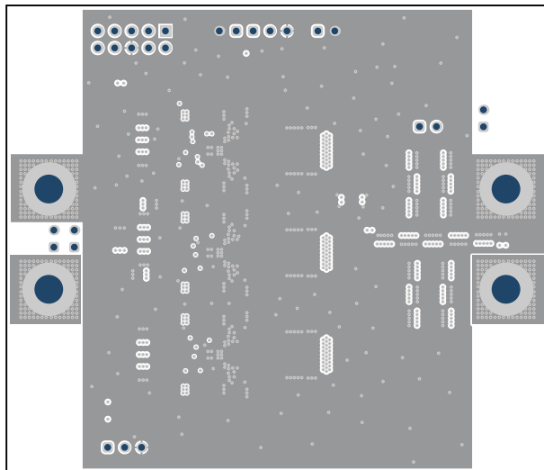
Figure 5-5. Layer 4
