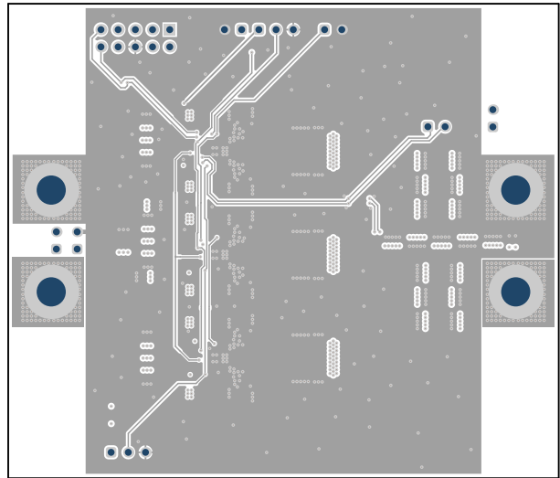
Figure 5-10. Layer 9
