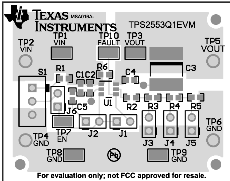
Figure 5. Layout—Top Composite
