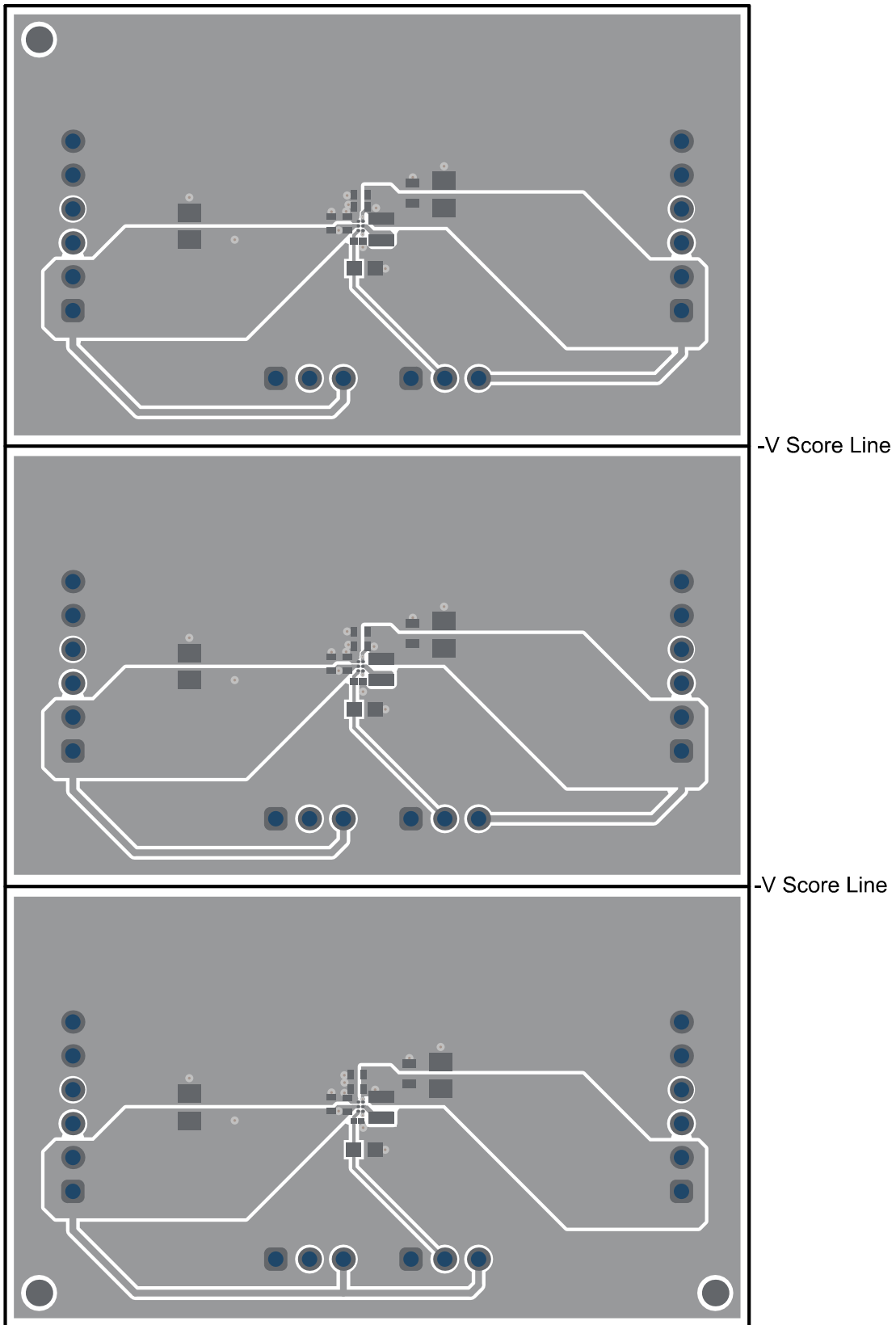
Figure 4. Top Layer
