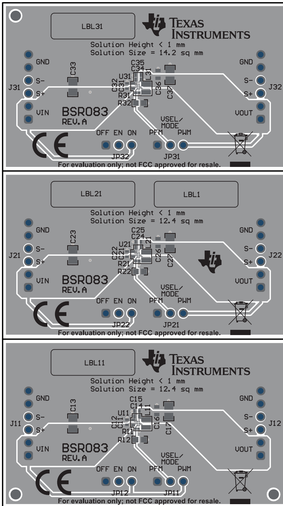
Figure 3. Top Assembly
