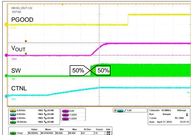
Figure 57. Start-Up Sequence
