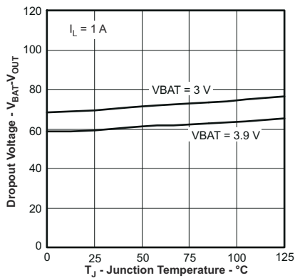
Figure 8-3. Dropout Voltage vs Temperature No Input Supply
