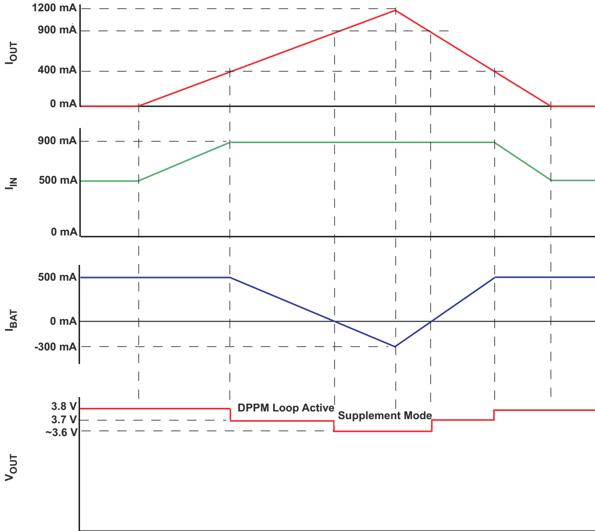
Figure 9-4. BQ24072 DPPM and Battery Supplement Modes ( V_{\text{OREG}} = V_{\text{BAT}} + 225 \text{ mV} , V_{\text{BAT}} = 3.6 \text{ V} )
