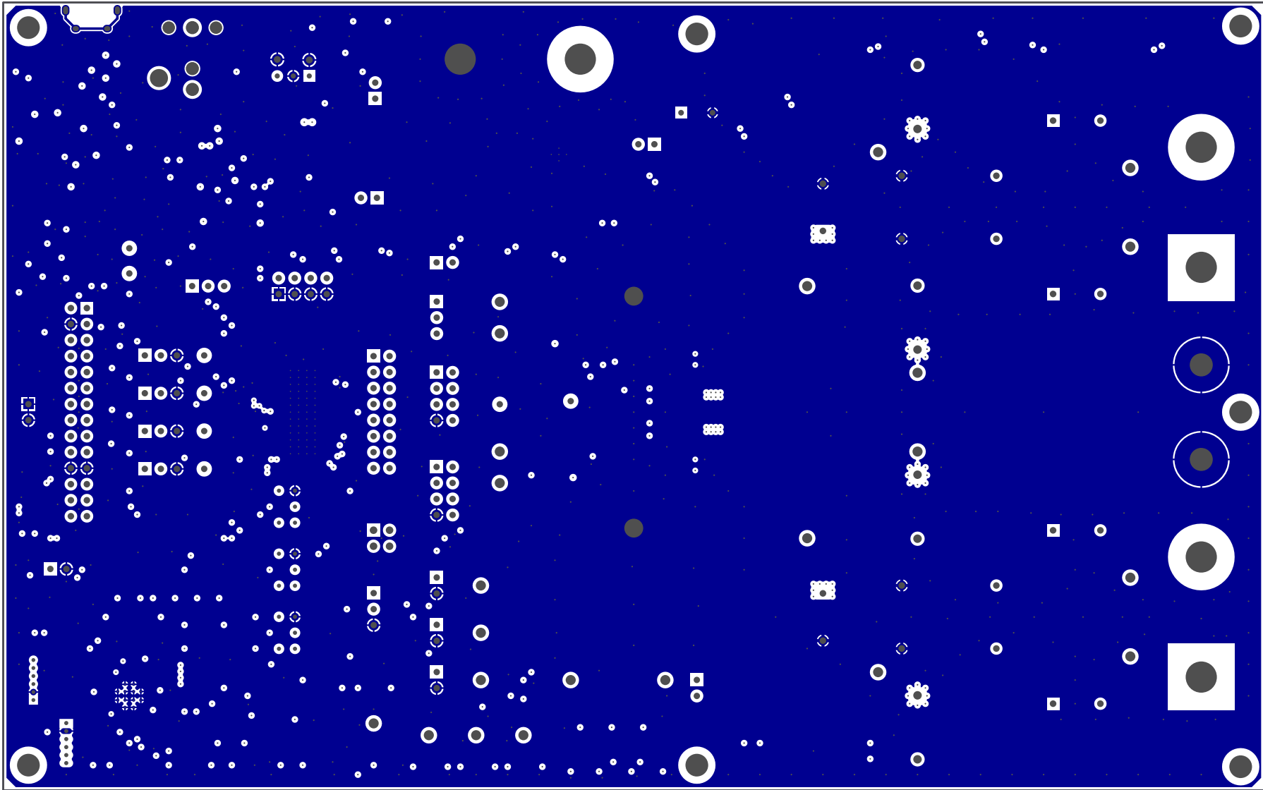
Signal Layer 1
