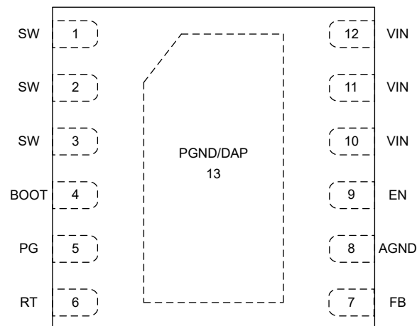
Figure 4-1. Pin Diagram
