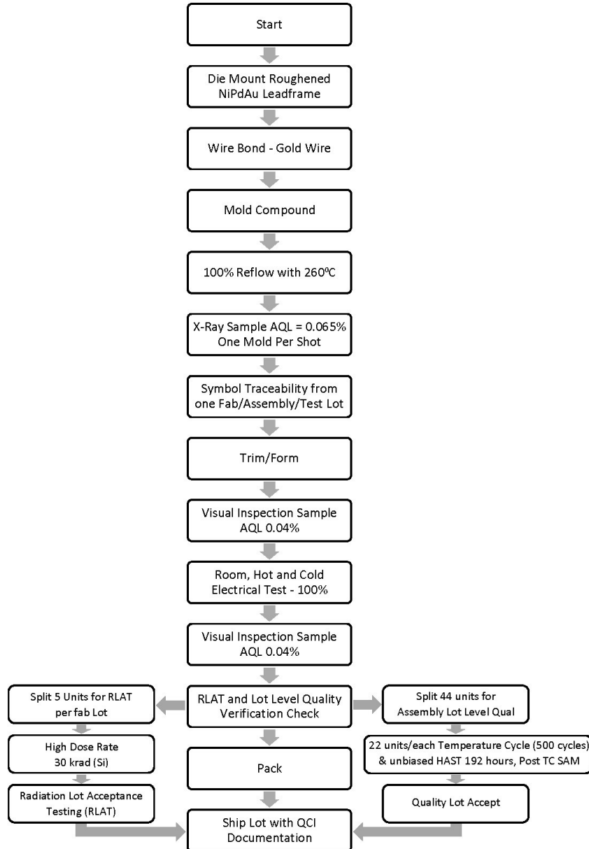
Figure 2-1. SN54SC3T97-SEP Space Enhanced Plastic Production Flow Chart
