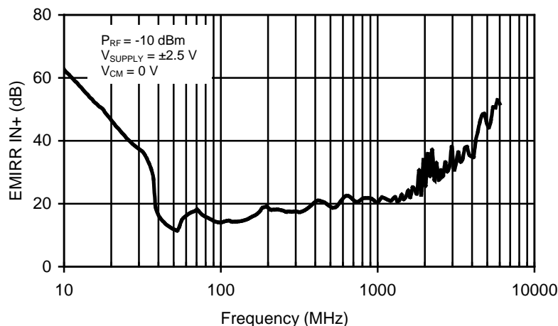
Figure 1. OPA354 EMIRR IN+ vs Frequency
