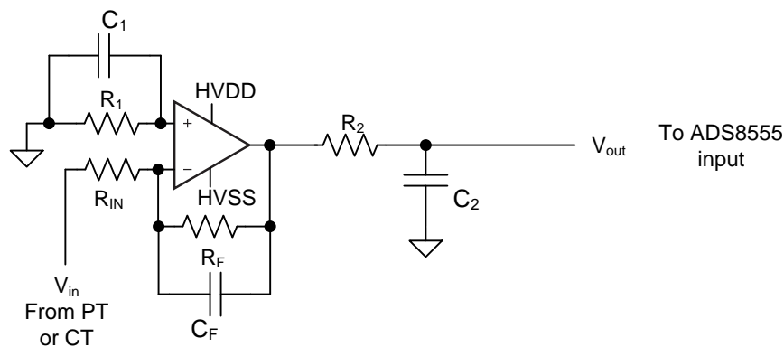
Figure 37. Op Amp in an Inverting Configuration
