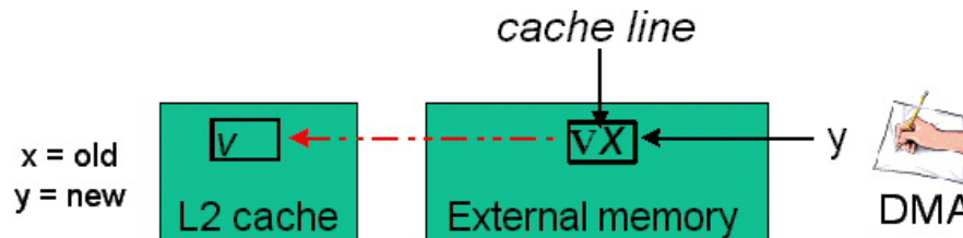
Figure 9. Cache Line Boundaries and the L2 Cache
