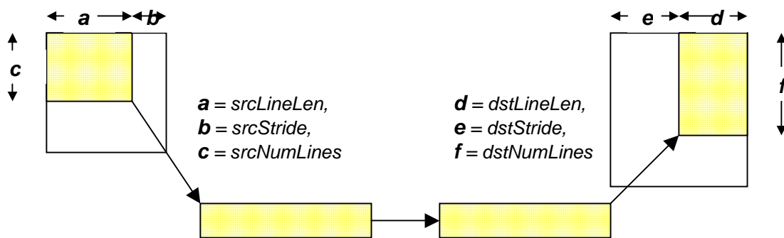
Figure 10. Illustration of FCPY doCopy operation
