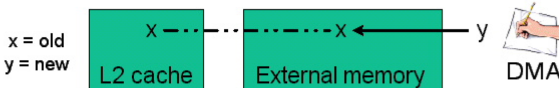
Figure 7. DMA Write Access Coherency Problem
