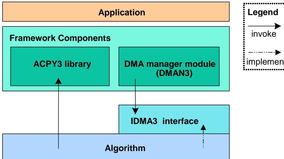
Figure 11. Dependencies in the fastcopytest Example
