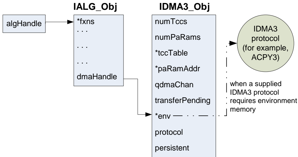
Figure 5. IDMA3 Logical Channels
