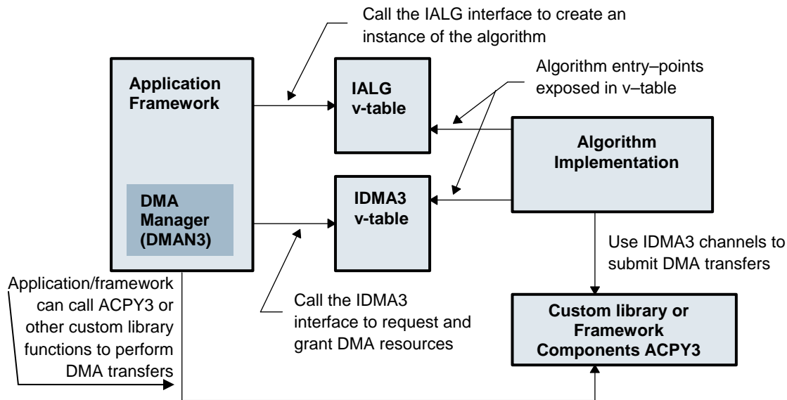
Figure 4. Algorithm Implementing IALG and IDMA3 Interfaces and Application Using Framework Components
