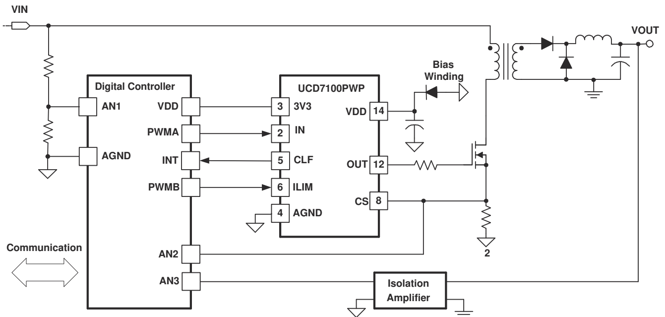
Figure 10-1. Typical Application
