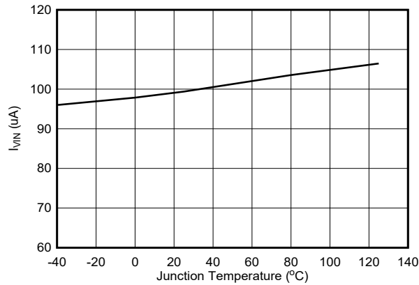
Figure 6-1. TPSM863252 Quiescent Current
