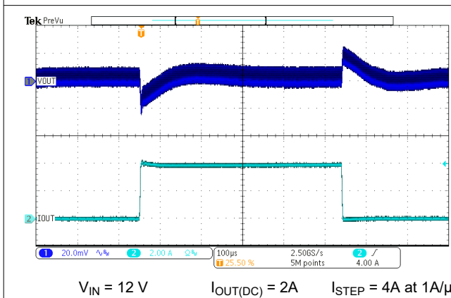
Figure 7-8. Load Transient
