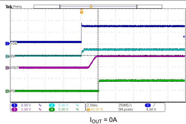
Figure 7-13. VIN Start-Up
