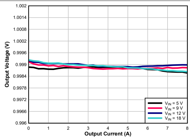
Figure 7-5. Load Regulation
