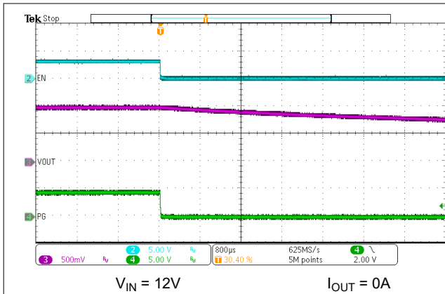
Figure 7-10. EN Shutdown No Load
