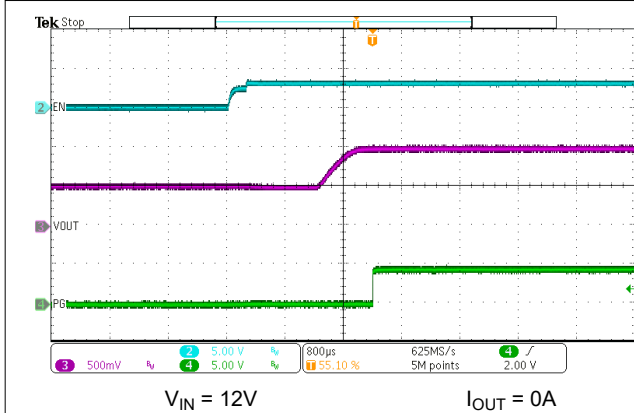
Figure 7-12. EN Start-Up – 0.5V Prebias
