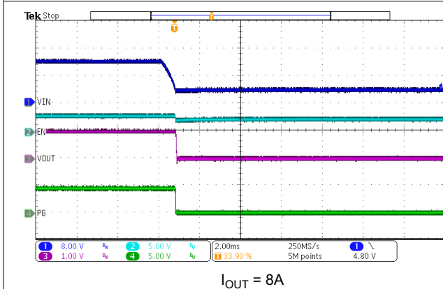
Figure 7-14. VIN Shutdown
