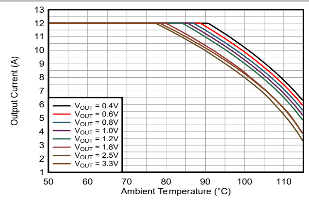
Figure 9-33. Safe Operating Area TPSM8287A12BAM V_{IN} = 5.0\text{V}
