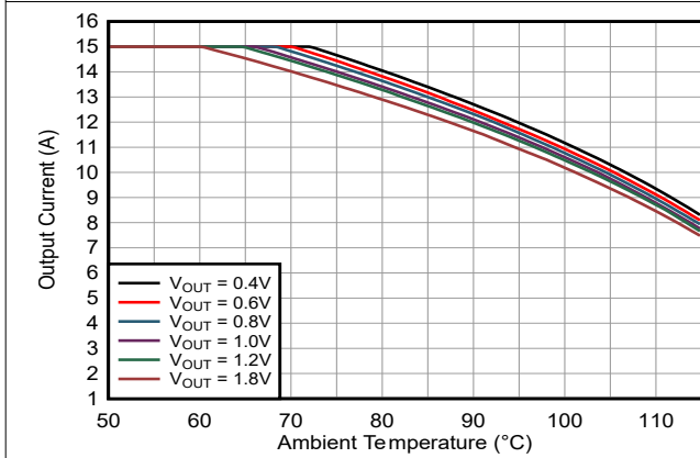
Figure 9-34. Safe Operating Area TPSM8287A12BBM V_{IN} = 3.3\text{V}
