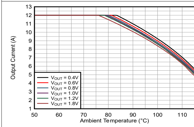
Figure 9-32. Safe Operating Area TPSM8287A12BAM V_{IN} = 3.3\text{V}
