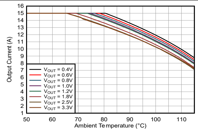
Figure 9-35. Safe Operating Area TPSM8287A12BBM V_{IN} = 5.0\text{V}
