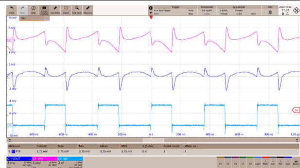
Figure 9-18. FPWM Operation I_{OUT} = 3A
