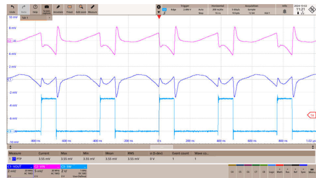
Figure 9-16. FPWM Operation I_{OUT} = 3A
