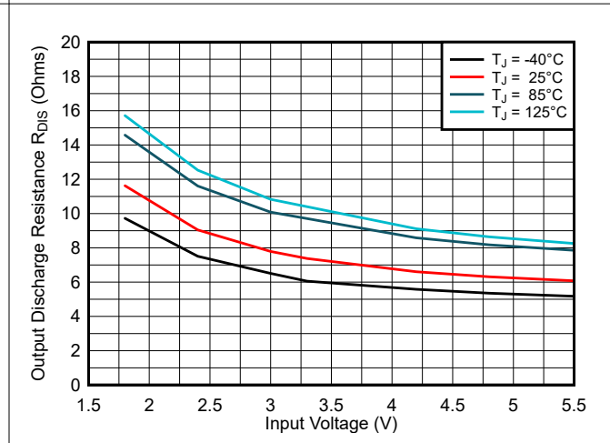
Figure 6-4. VOS Discharge Switch Drain Source Resistance R_{DIS}
