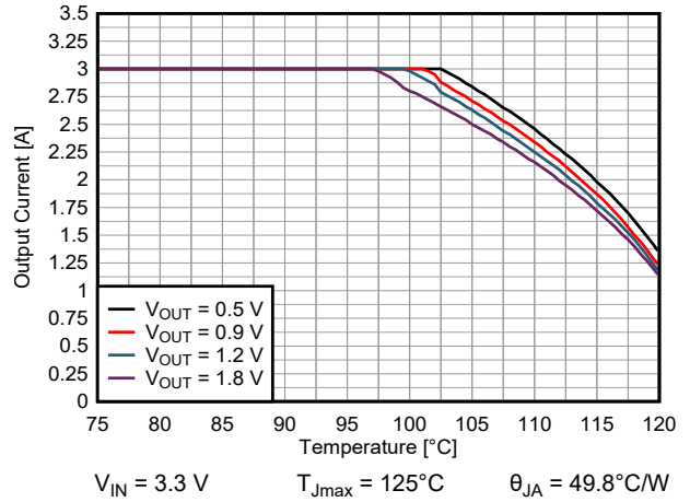
Figure 8-33. Thermal Derating (Safe Operating Area)
