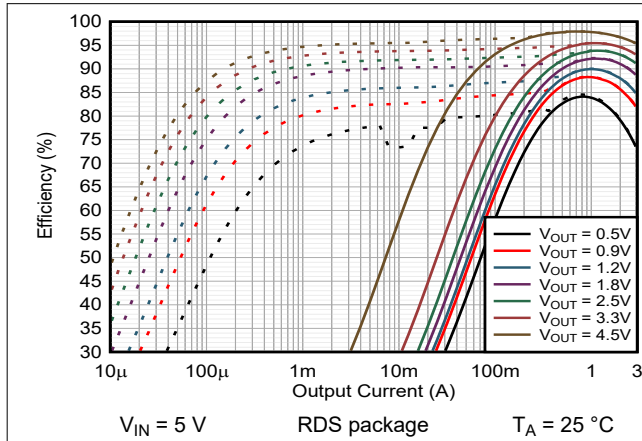
Figure 8-2. Efficiency versus Output Current
