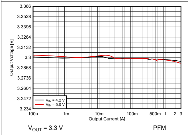
Figure 8-24. Output Voltage versus Output Current
