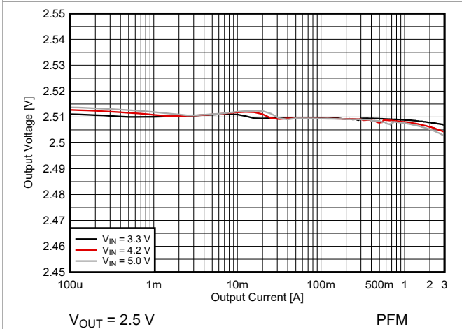
Figure 8-22. Output Voltage versus Output Current
