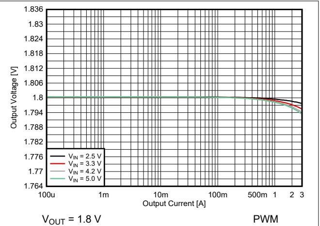
Figure 8-21. Output Voltage versus Output Current
