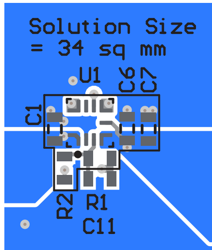
Figure 8-49. PCB Layout Recommendation (VCB Package)
