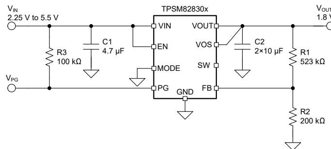
Figure 8-1. Typical Application of TPSM82830x
