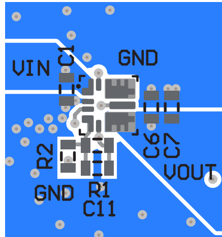
Figure 8-48. PCB Layout Recommendation (RDS Package)
