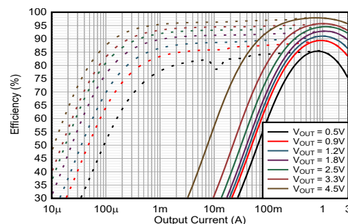
Efficiency at V IN = 5V, VCB Package
