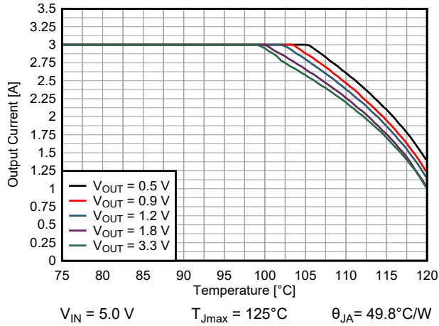
Figure 8-32. Thermal Derating (Safe Operating Area)
