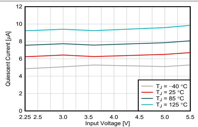
Figure 6-4. Quiescent Current
