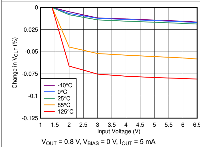
Figure 6-29. Line Regulation Without Bias
