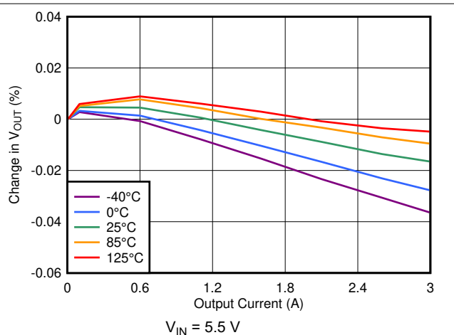
Figure 6-28. Load Regulation (5-V Output)
