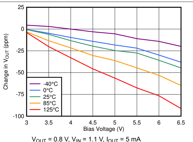
Figure 6-30. Line Regulation Without Bias
