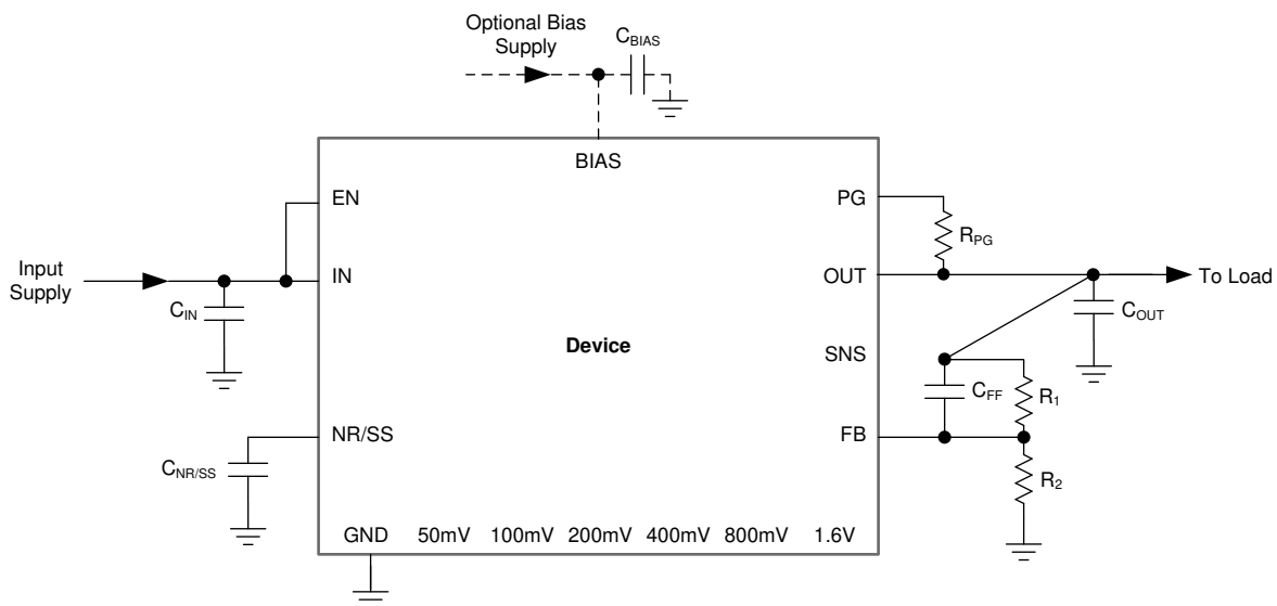
Figure 8-23. Typical Application
