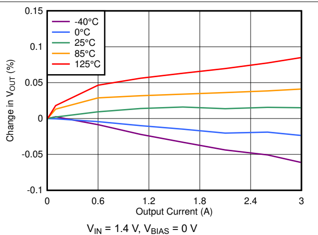
Figure 6-26. Load Regulation With Bias
