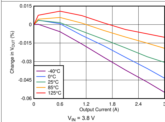
Figure 6-27. Load Regulation (3.3-V Output)
