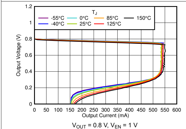
Figure 5-45. Current Limit
