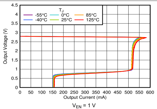
Figure 5-44. Current Limit
