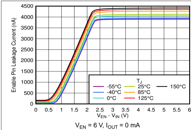
Figure 5-43. Enable Pin Leakage Current vs V_{EN} - V_{IN}
