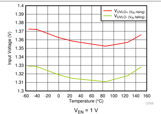
Figure 5-46. UVLO Threshold vs Temperature
