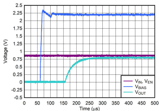
Figure 6-17. Start-Up With V_{\text{IN}} and V_{\text{EN}} Before V_{\text{BIAS}}
