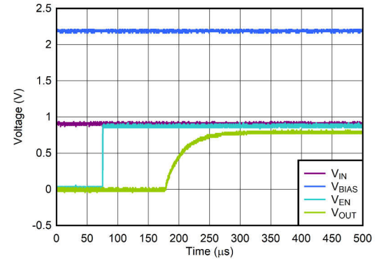
Figure 6-16. Start-Up With V_{\text{IN}} and V_{\text{BIAS}} Before V_{\text{EN}}
