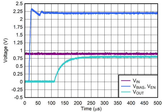
Figure 6-15. Start-Up With V_{\text{IN}} Before V_{\text{BIAS}} and V_{\text{EN}}
