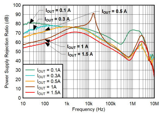
Figure 5-18. V_{IN} PSRR vs Frequency
