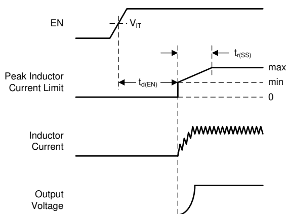
Figure 15. Device Start-Up
