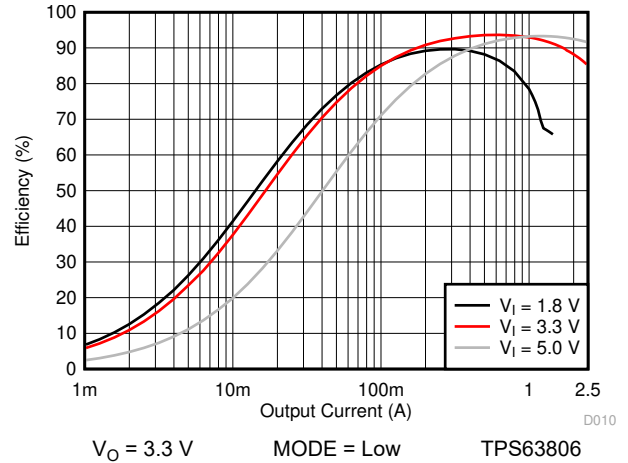
Figure 10-16. Efficiency versus Input Voltage (PWM Only)
