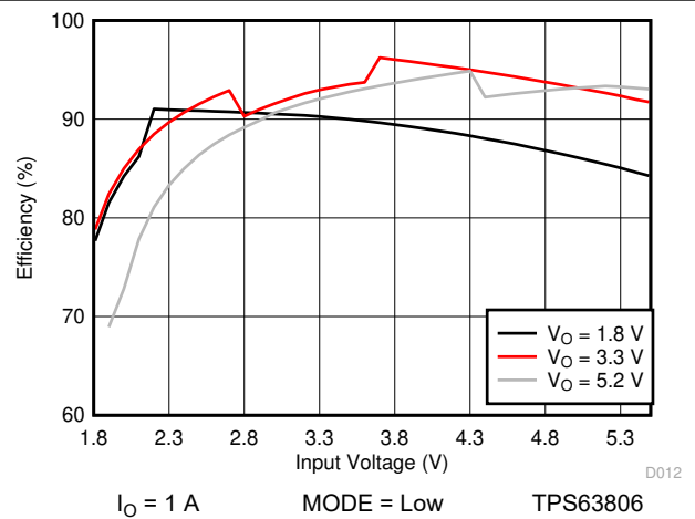
Figure 10-18. Efficiency versus Input Voltage (PWM Only)
