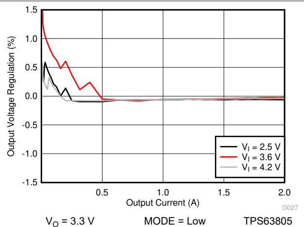
Figure 10-20. Load Regulation (PFM/PWM)
