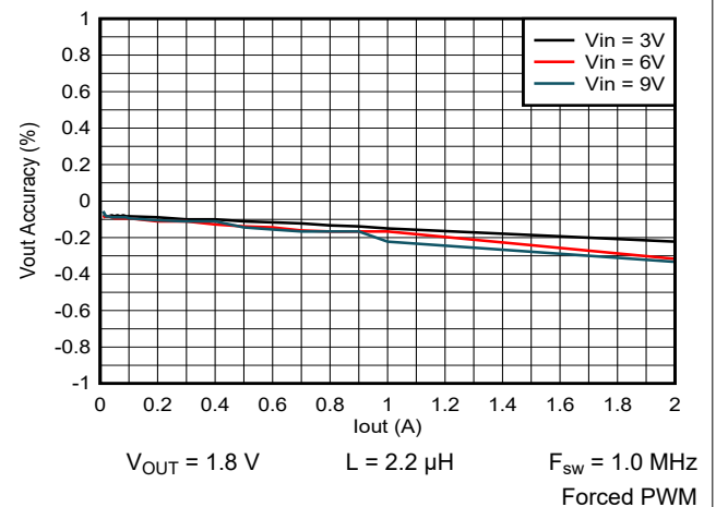
Figure 9-14. Output Voltage vs Output Current
