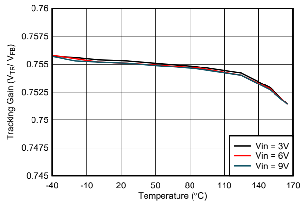
Figure 7-10. Tracking Voltage Gain vs Temperature
