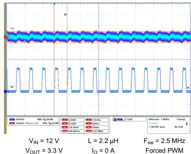
Figure 9-73. Output Voltage Ripple
