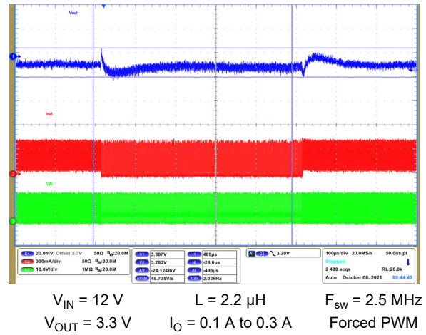
Figure 9-71. Load Transient Response
