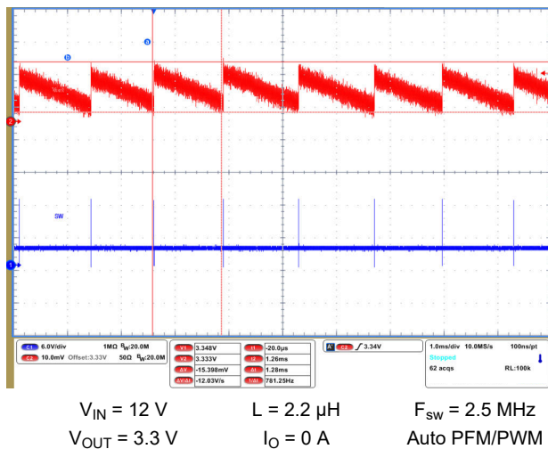
Figure 9-72. Output Voltage Ripple
