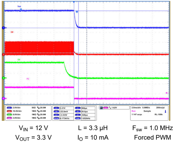
Figure 9-68. Shutdown Timing with Output Discharge Enabled
