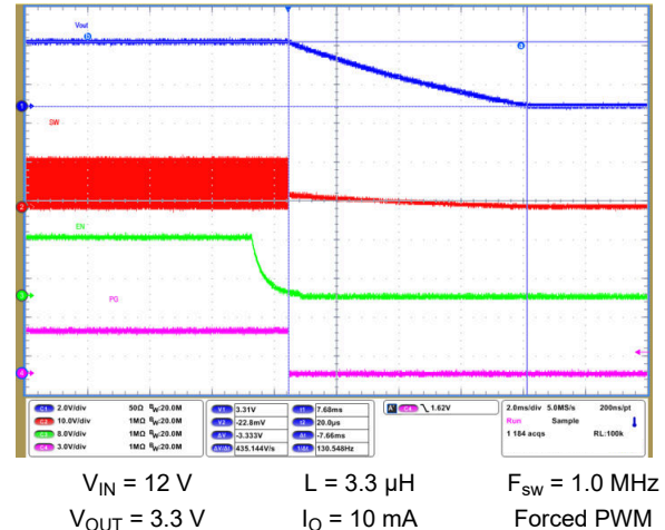
Figure 9-69. Shutdown Timing with Output Discharge Disabled
