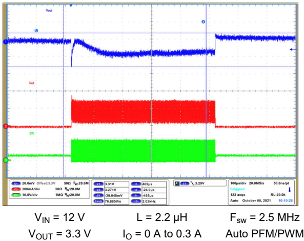
Figure 9-70. Load Transient Response
