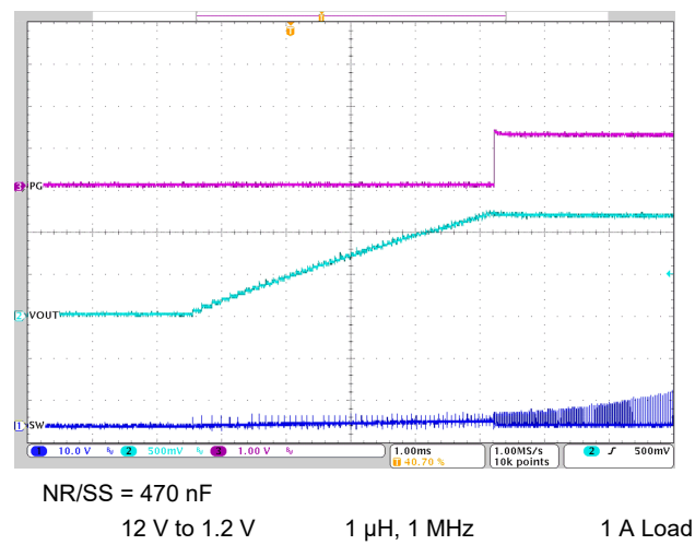
Figure 7-10. Start-up
