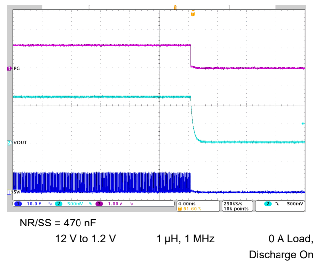
Figure 7-11. Shutdown
