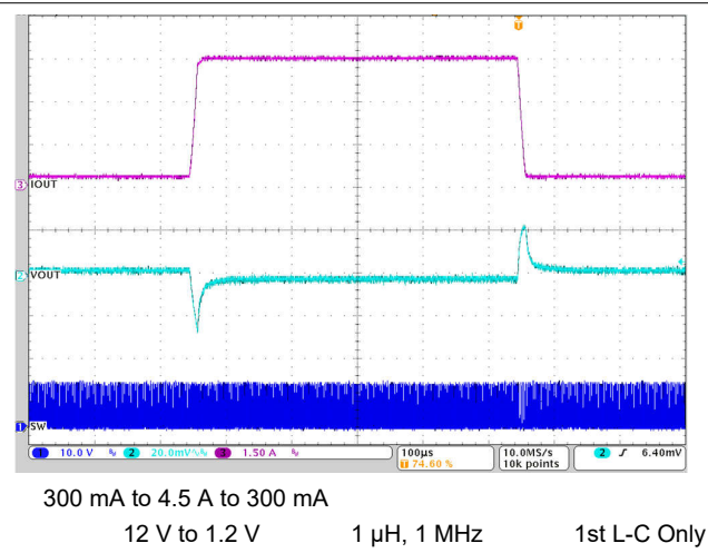
Figure 7-12. Load Transient
