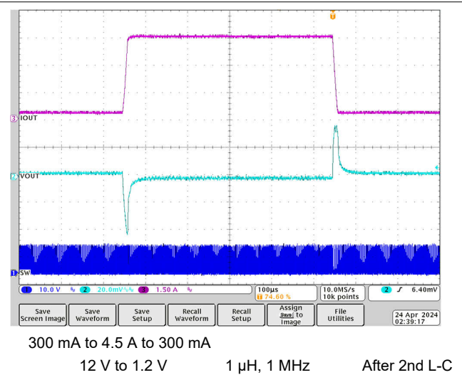
Figure 7-13. Load Transient
