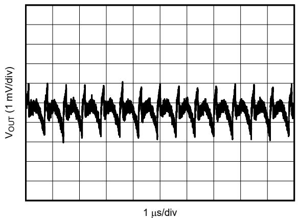
Figure 5-5. V_{OUT} Ripple After the First L-C Filter
