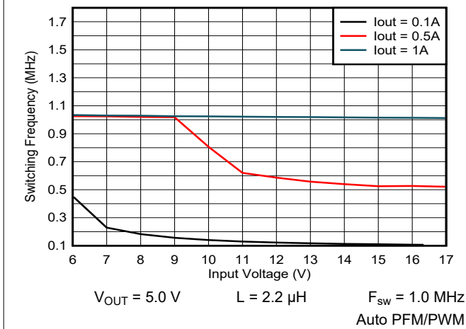
Figure 9-48. Switching Frequency vs Input Voltage
