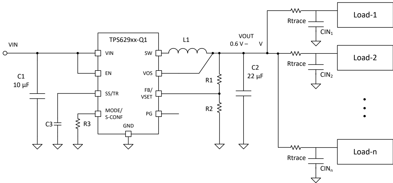
Figure 9-65. Multiple Loads
