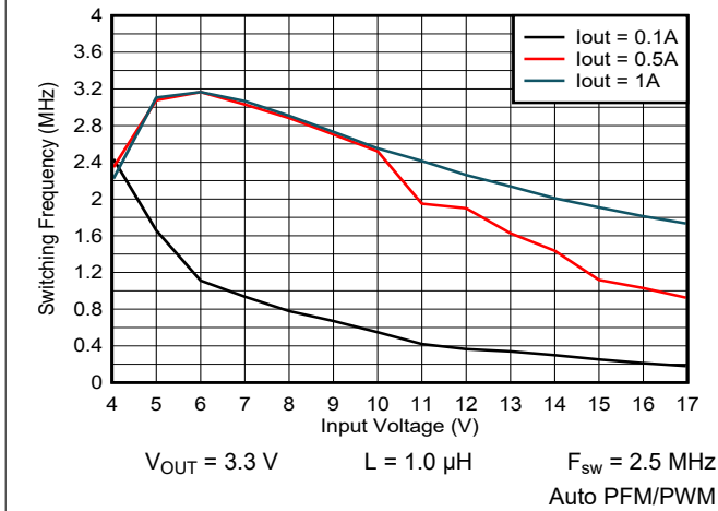
Figure 9-54. Switching Frequency vs Input Voltage
