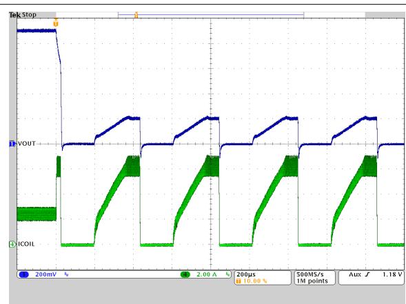
Figure 9-19. HICCU Protection
