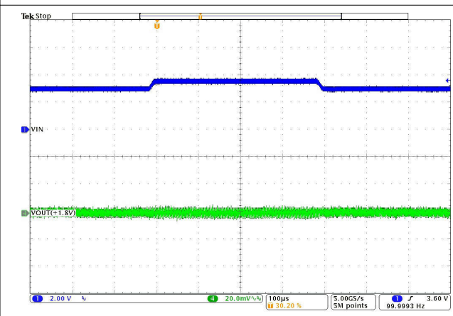
Figure 8-36. Line Transient
