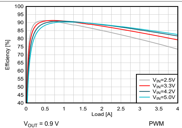
Figure 8-12. Efficiency versus Output Current
