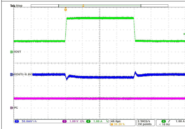
Figure 8-33. Load Transient
