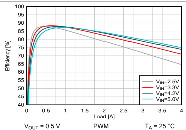
Figure 8-14. Efficiency versus Output Current
