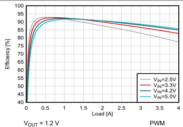
Figure 8-10. Efficiency versus Output Current
