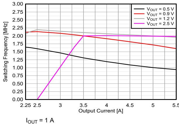
Figure 8-29. Switching Frequency versus Input Voltage I OUT = 1 A
