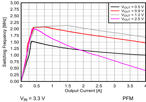
Figure 8-27. Switching Frequency versus Output Current V IN = 3.3 V PFM
