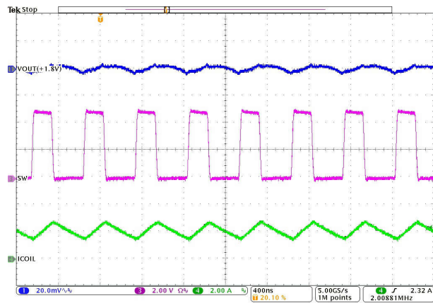
I OUT = 2.0 A PFM or PWM Figure 8-31. Output Voltage Ripple
