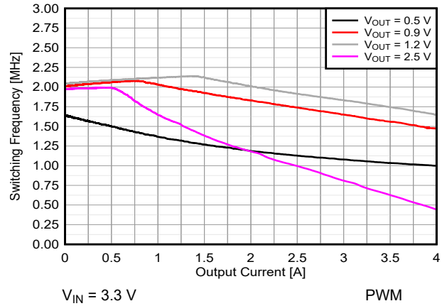
Figure 8-28. Switching Frequency versus Output Current V IN = 3.3 V PWM
