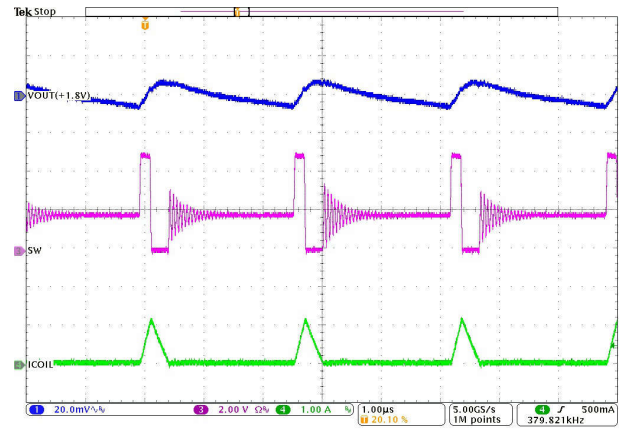
I OUT = 100 mA PFM Figure 8-30. Output Voltage Ripple
