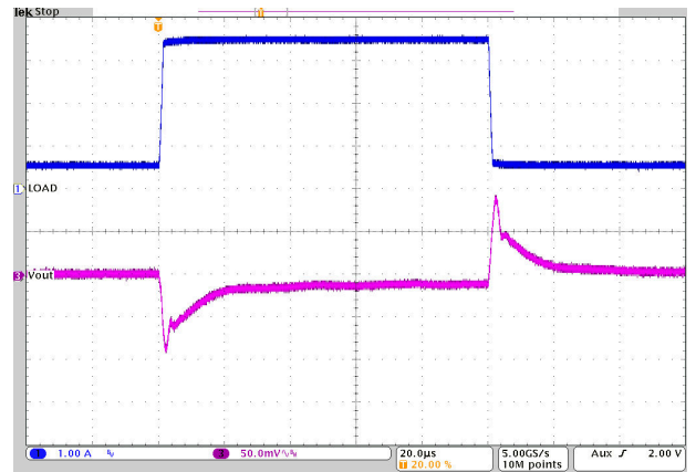
V_{OUT} = 1.2V PWM T_A = 25^\circ C V_{IN} = 5.0V I_{OUT} = 0.4A \text{ to } 3.6A \text{ to } 0.4A
