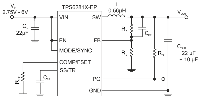
Figure 7-2. Measurement Setup for TPS62811-EP (1A) and TPS62812-EP (2A)
