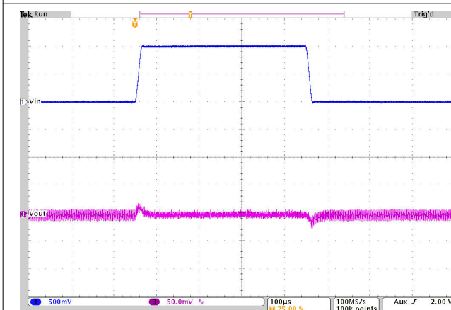
V_{OUT} = 1.2V PFM T_A = 25^\circ C I_{OUT} = 0.5A V_{IN} = 4.5V \text{ to } 5.5V \text{ to } 4.5V
