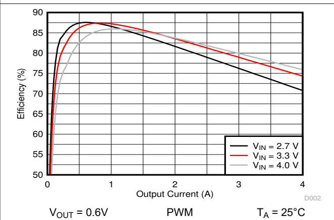
Figure 9-11. Efficiency versus Output Current
