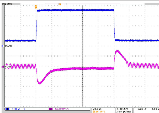
Figure 9-22. Load Transient Response
