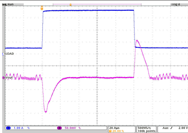
Figure 9-20. Output Voltage versus Output Current
