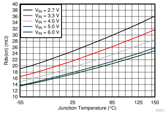
Figure 6-2. R_{ds(on)} of Low-side Switch
