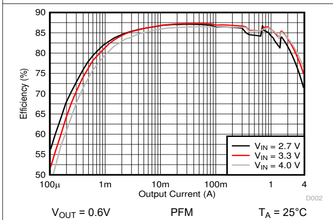
Figure 9-10. Efficiency versus Output Current
