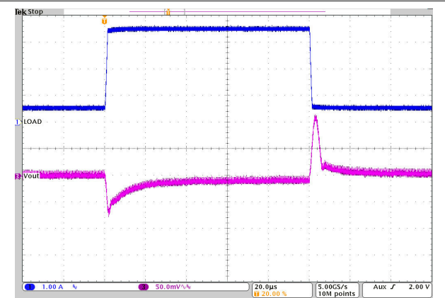
V_{OUT} = 1.0V PWM T_A = 25^\circ C V_{IN} = 5.0V I_{OUT} = 0.4A \text{ to } 3.6A \text{ to } 0.4A
