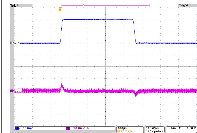
V_{OUT} = 1.8V PFM T_A = 25^\circ C I_{OUT} = 0.5A V_{IN} = 4.5V \text{ to } 5.5V \text{ to } 4.5V
