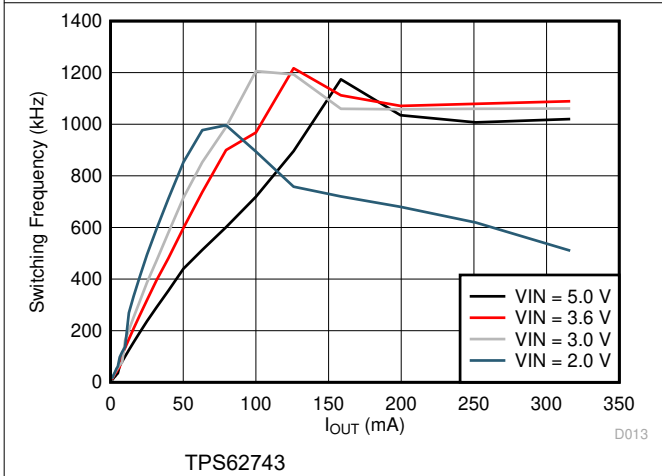
Figure 9-12. Switching Frequency vs Load Current V_{OUT} = 1.2\text{ V}
