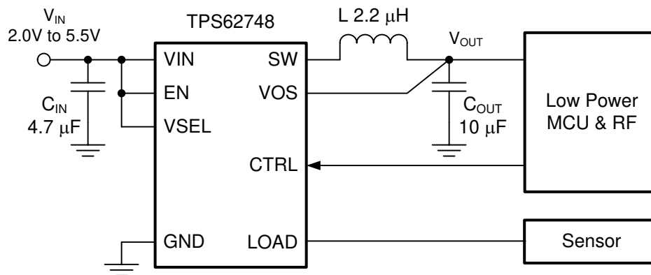
Figure 9-1. TPS62748 Typical Application Circuit
