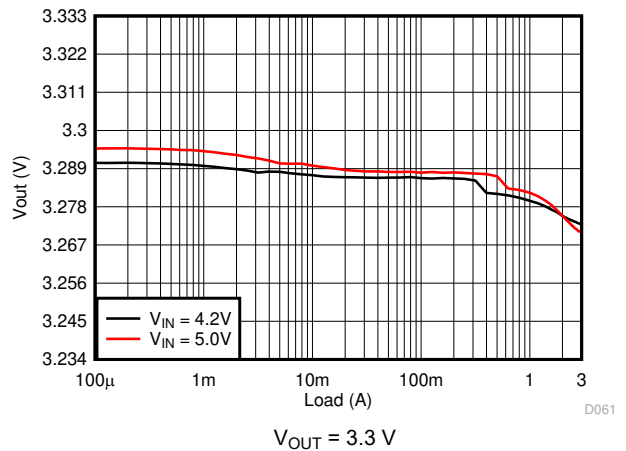
Figure 8-20. Load Regulation
