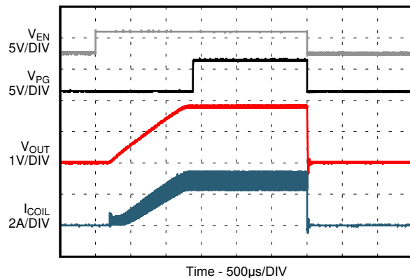
Figure 8-30. Start-Up With No Load
