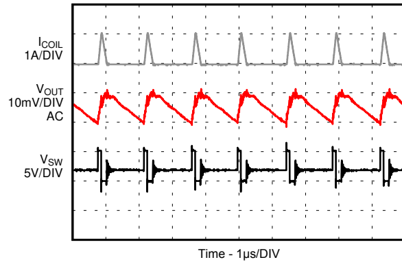
Figure 8-28. PSM Operation
