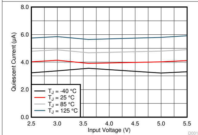
Figure 6-3. Quiescent Current
