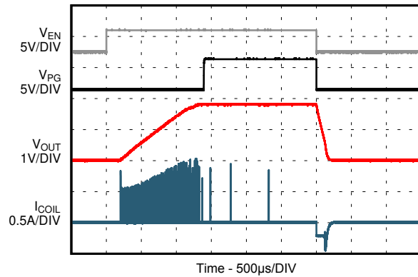
Figure 8-28. PSM Operation
