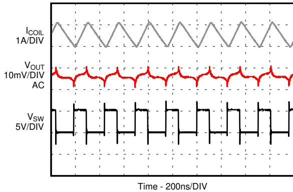
Figure 8-27. PWM Operation
