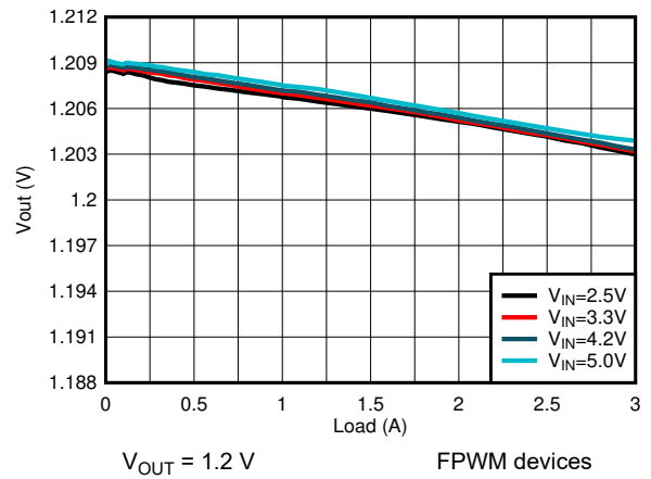
Figure 8-14. Load Regulation
