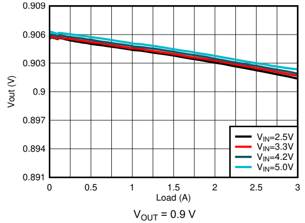
Figure 8-10. Load Regulation
