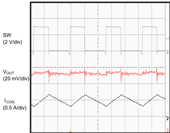
Figure 23. Typical Application (PWM Mode) VIN = 3.3 V, VOUT = 1.2 V, Load Current = 500 mA
