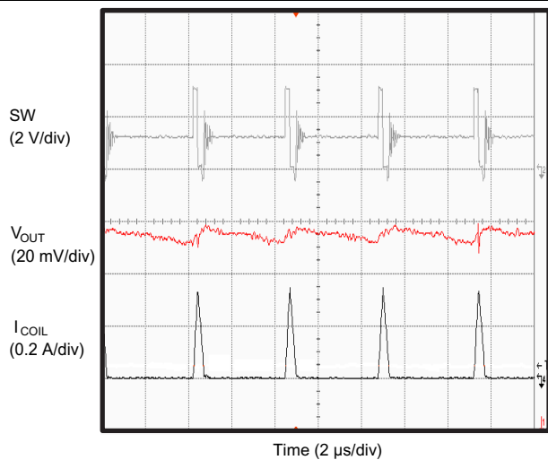
Figure 24. Typical Application (PFM Mode) VIN = 3.3 V, VOUT = 1.2 V, Load Current = 10 mA
