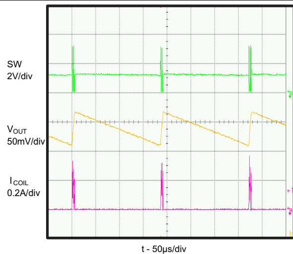
Figure 25. Typical Application (Snooze Mode) VIN = 3.3 V, VOUT = 1.2 V, Load Current = 2 mA
