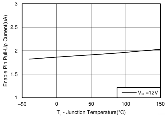
Figure 5-7. Enable Pullup Current, V EN = 1.0 V
