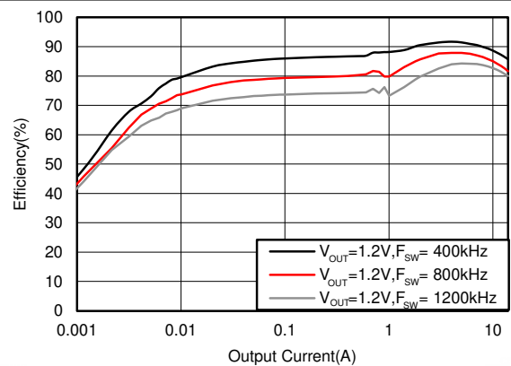
Figure 5-12. Efficiency with External VREG5 = 5 V, V IN = 12 V
