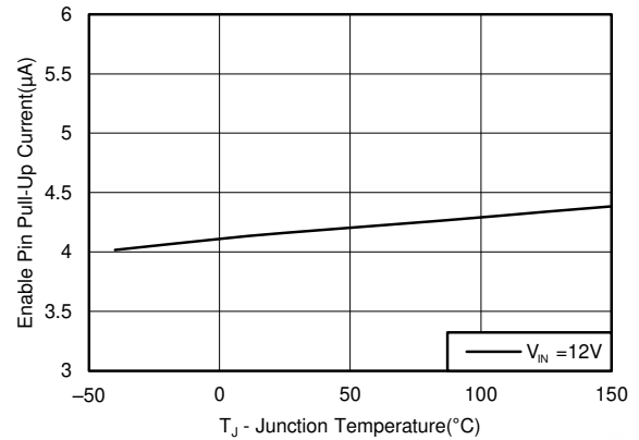
Figure 5-8. Enable Pullup Current, V EN = 1.3 V
