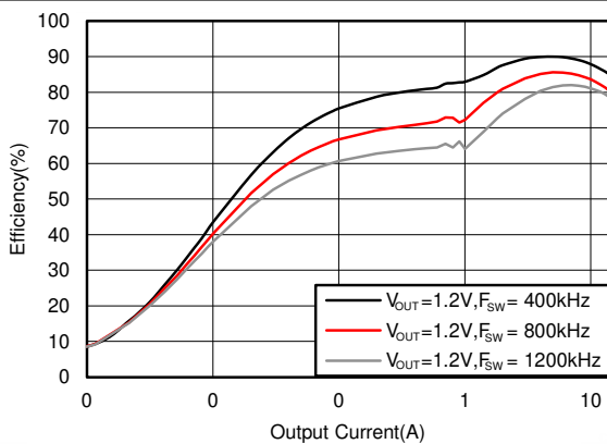
Figure 5-11. Efficiency with Internal VREG5 = 4.7 V, V IN = 12 V
