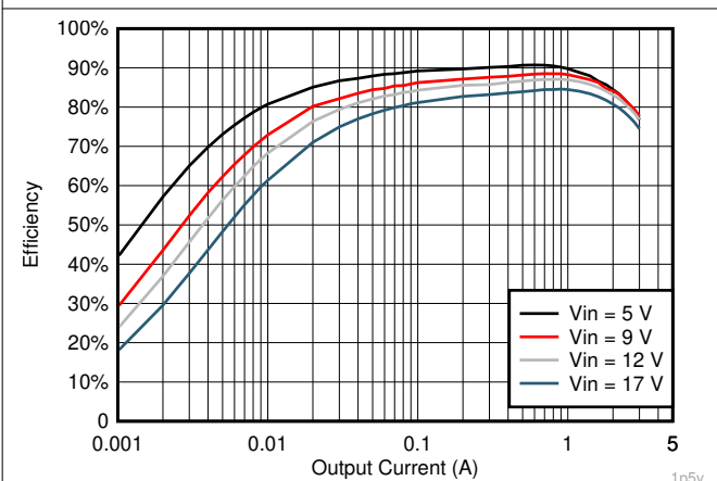
Figure 6-11. V_{OUT} = 1.5\text{ V} Efficiency, L = 1.5\ \mu\text{H}
