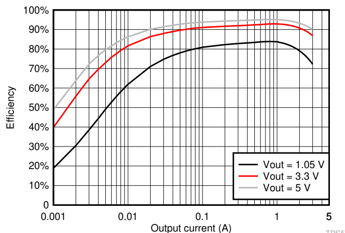
TPS563202 Efficiency
