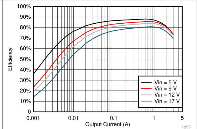
Figure 6-10. V_{OUT} = 1.05\text{ V} Efficiency, L = 1.2\ \mu\text{H}
