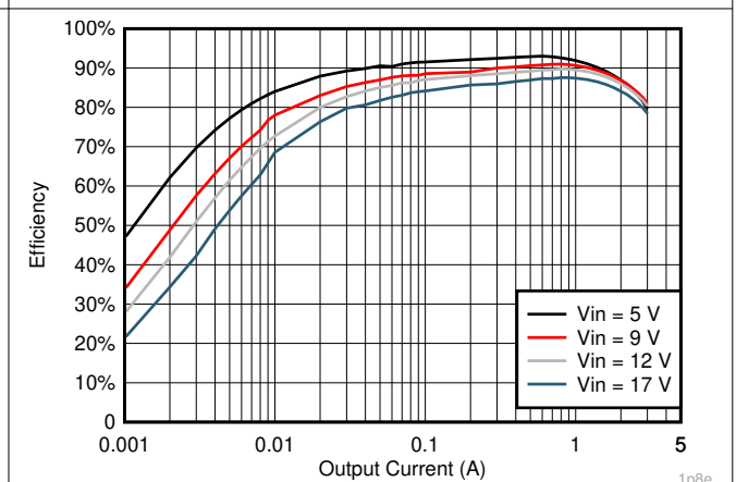
Figure 6-12. V_{OUT} = 1.8\text{ V} Efficiency, L = 2.2\ \mu\text{H}
