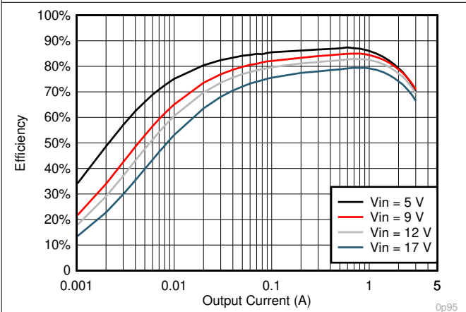
Figure 6-9. V_{OUT} = 0.95\text{ V} Efficiency, L = 1.2\ \mu\text{H}
