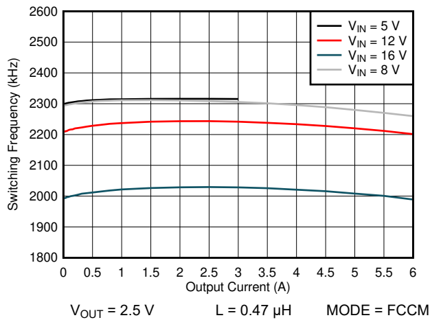
Figure 5-17. 2200 kHz Switching Frequency vs Load Current
