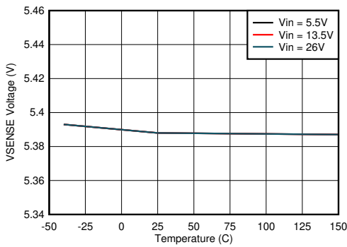
Figure 8-5. V_{SENSE} Voltage vs Junction Temperature
