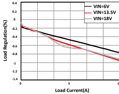
Figure 11-5. Load Regulation
